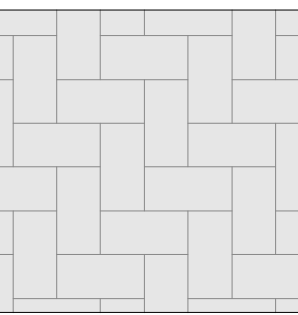
Porcelain Ground Paving: Herringbone W600 X L300 X D20MM
