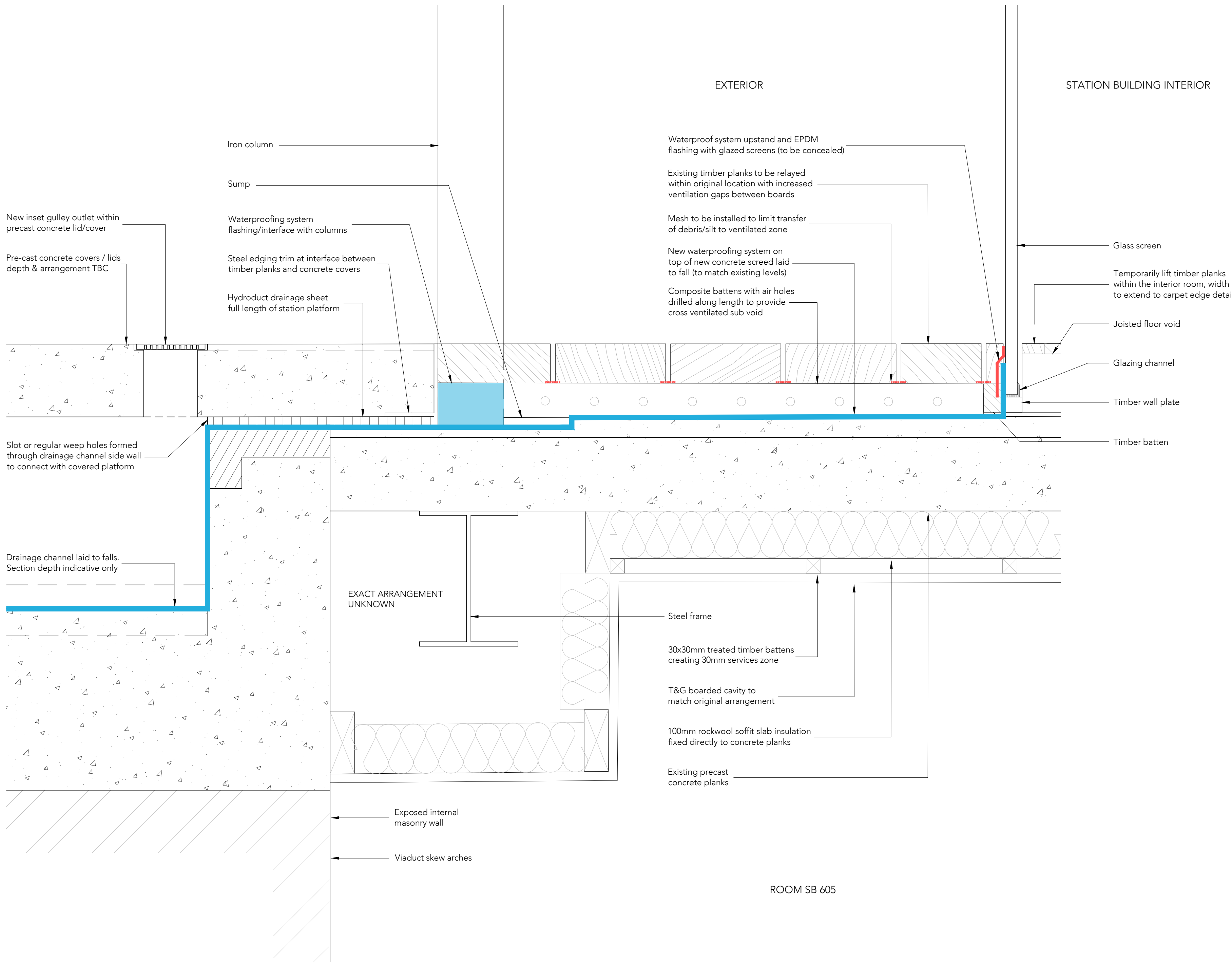
Typical Detail Through Glass Screen F-F as Proposed Scale 1:5
