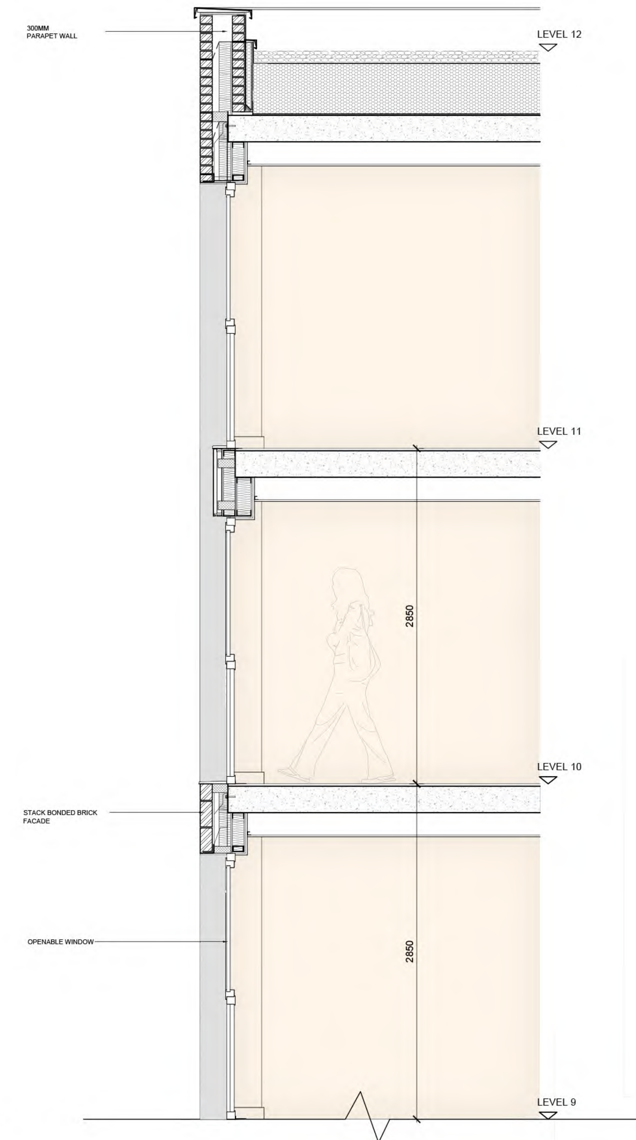
EXTERNAL WALL DETAIL SECTION C-1
