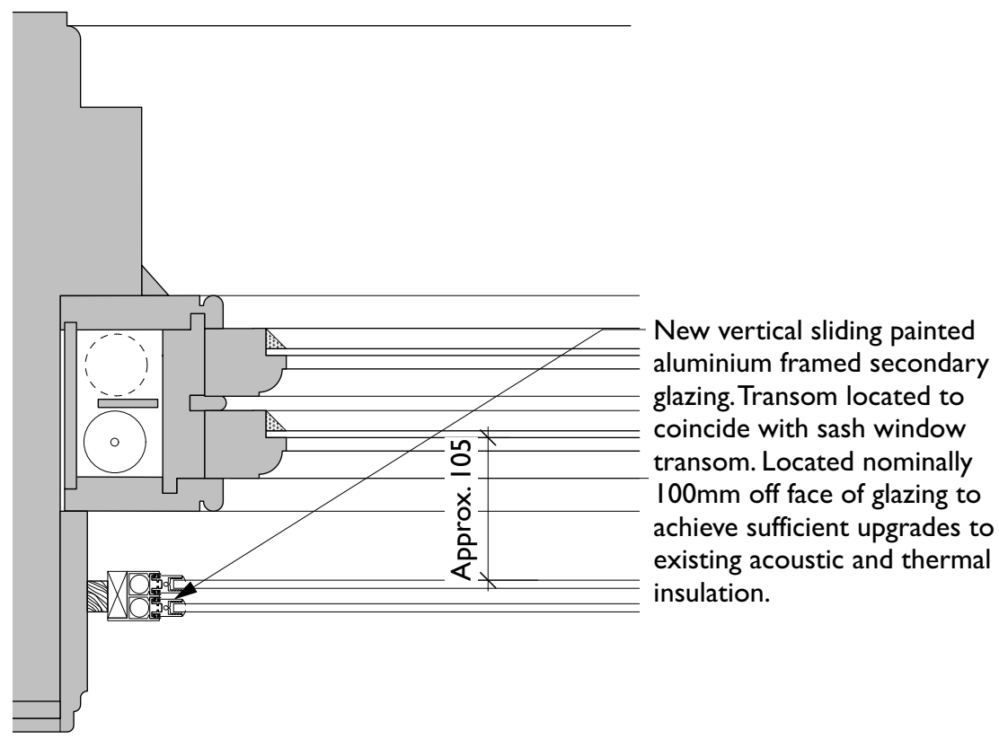
2 Typical Window Reveal - Secondary Glazing Scale: 1:5
