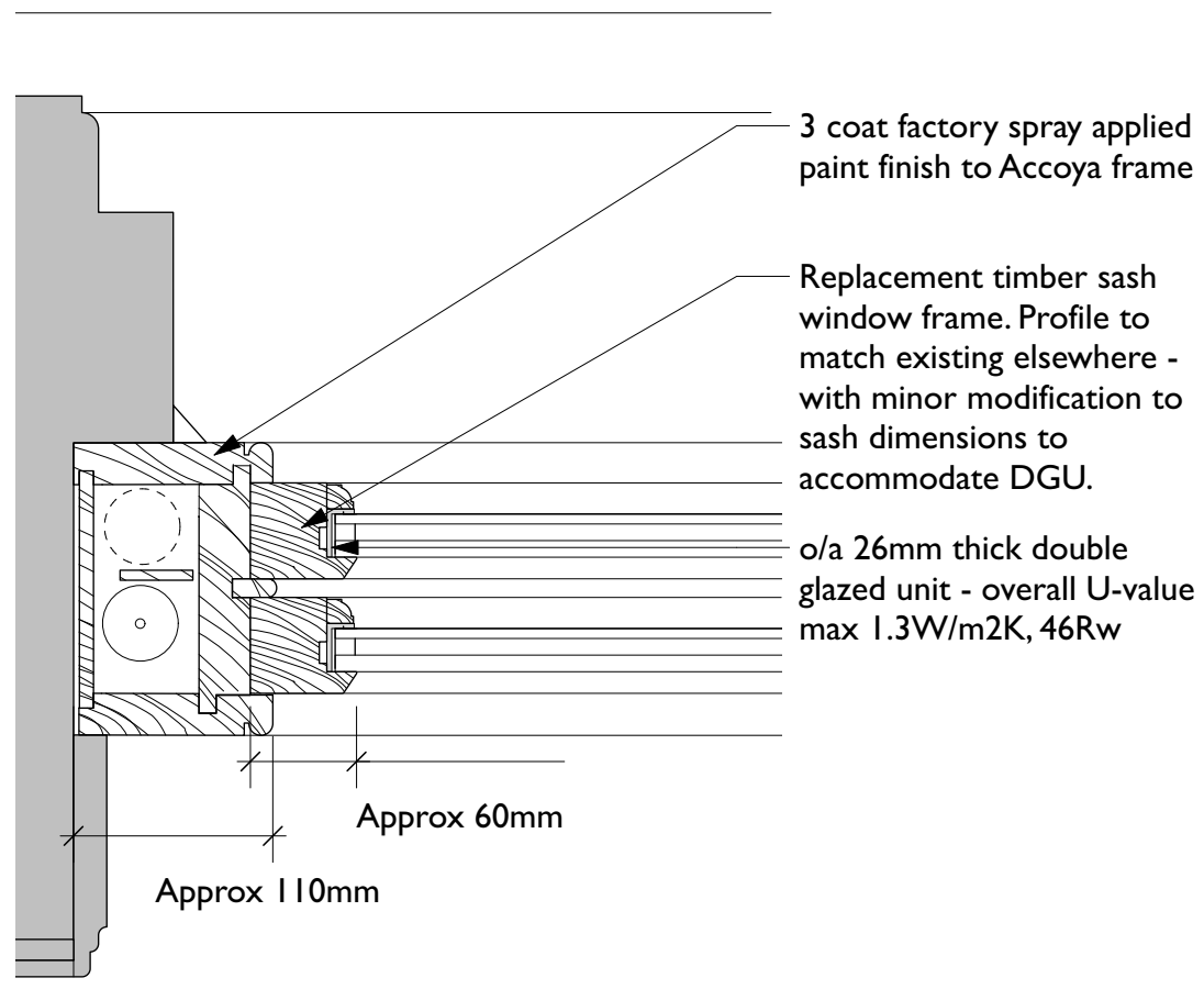
1 Typical Window Reveal - Replacement Sash Scale: 1:5
