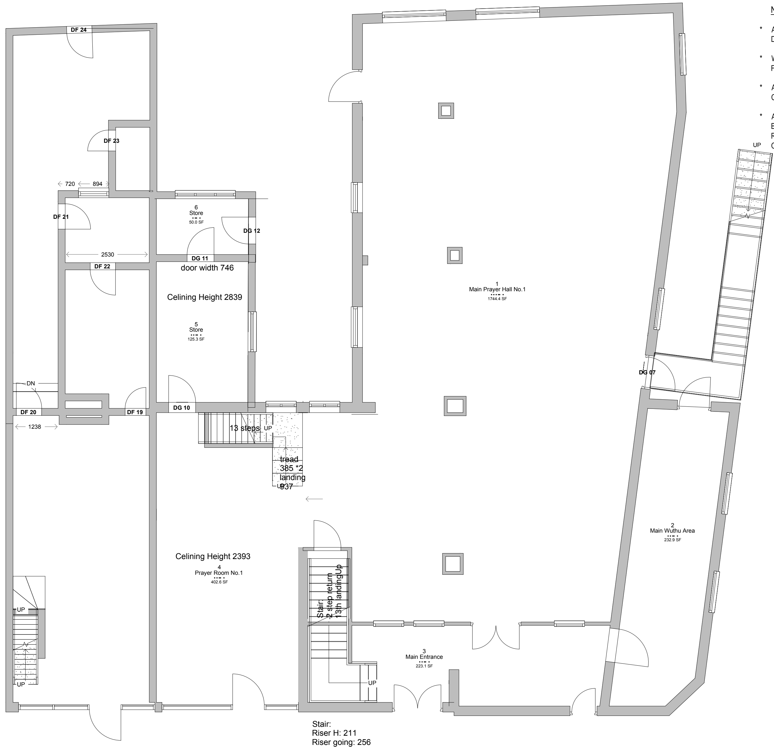
EXISTING GROUND FLOOR LAYOUT PLAN SCALE 1:100
