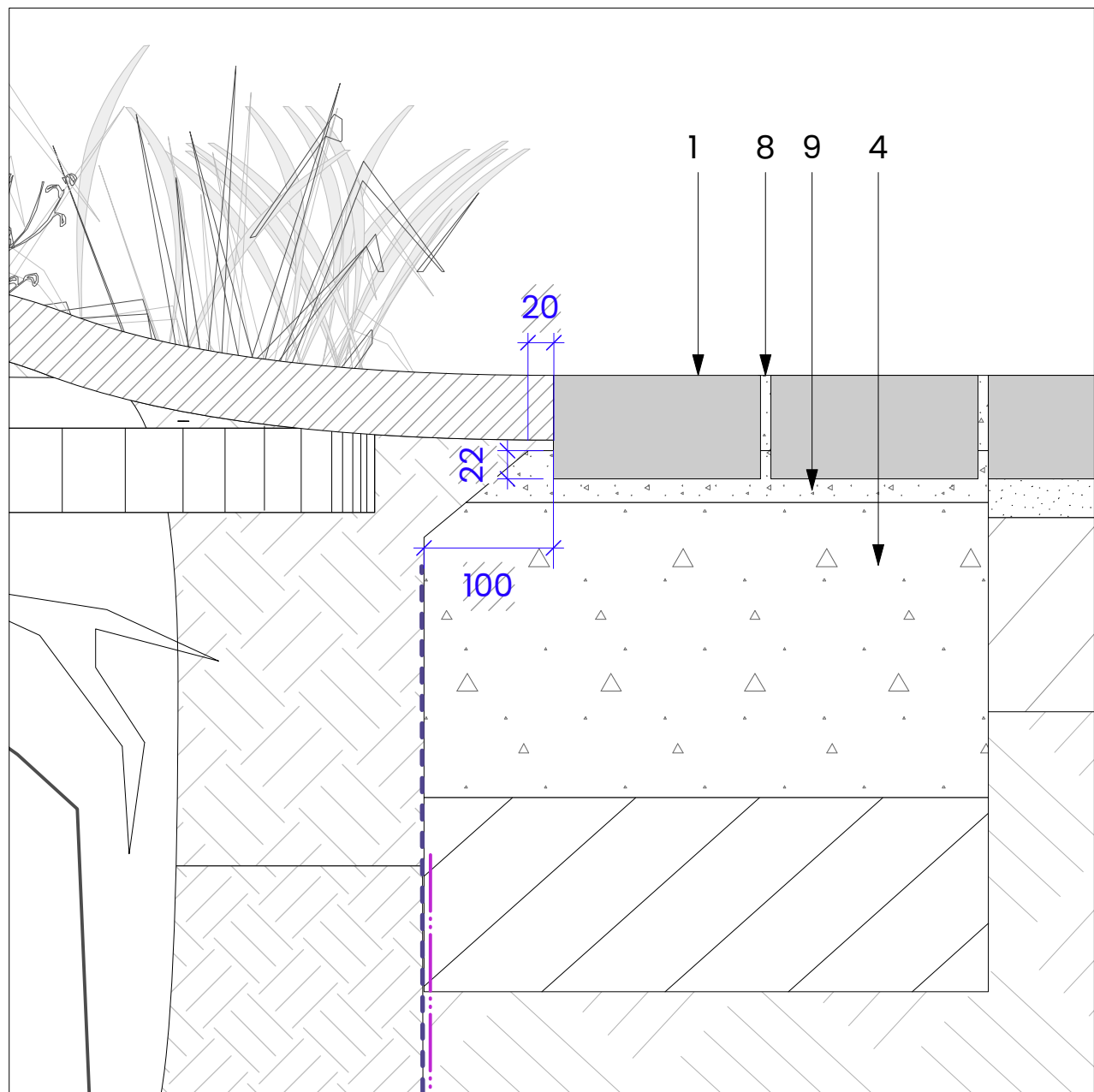
D02 Concrete Haunch Design Intent Scale: 1:5 @ A1
