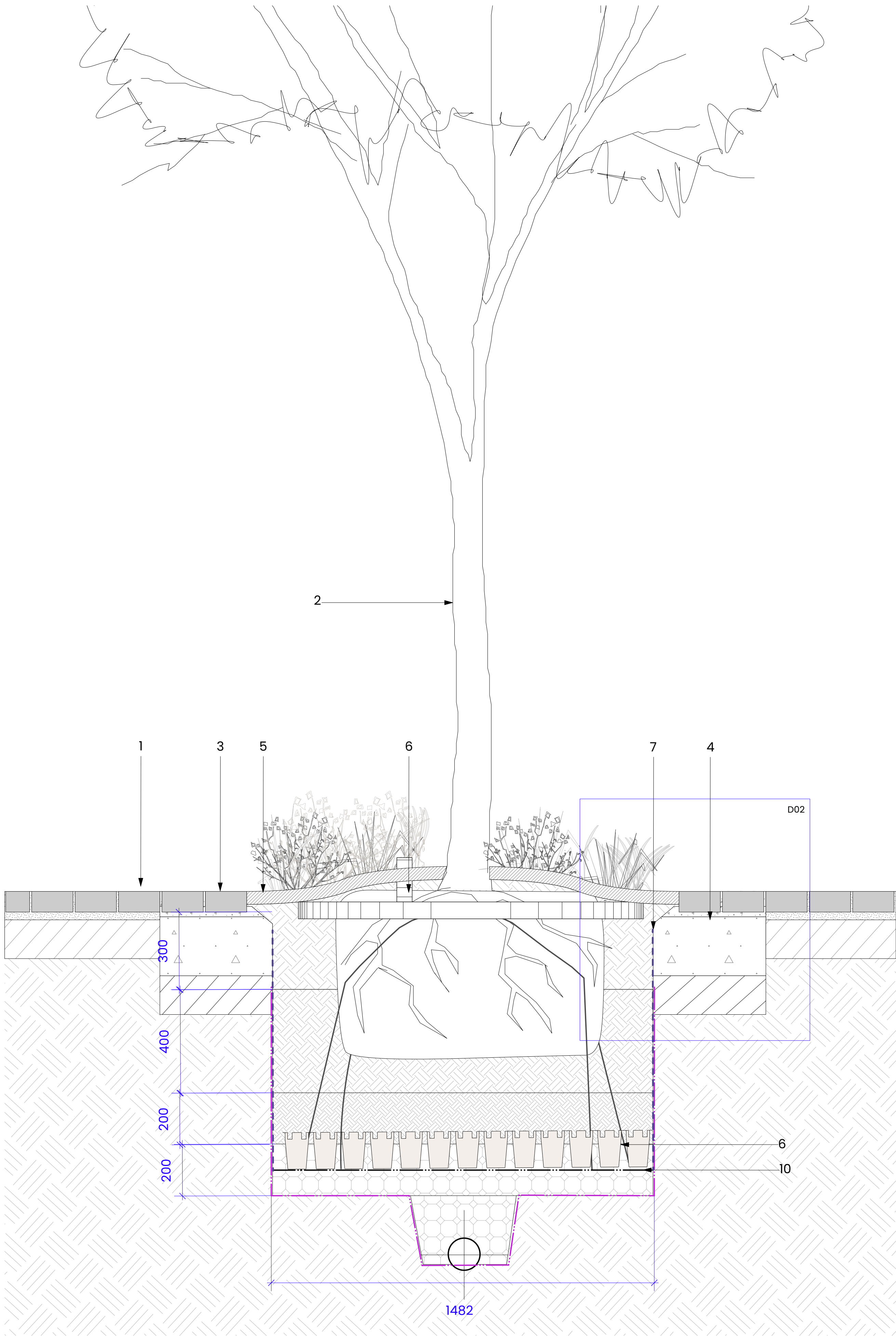
D01 Typical Tree Pit Adjacent to Driveway Scale: 1:10 @ A1
