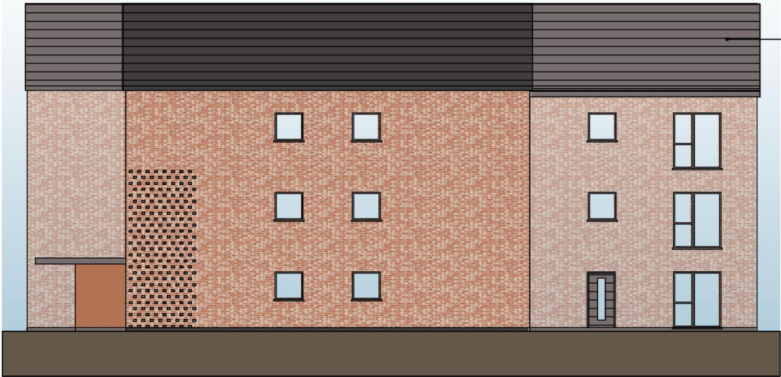
Proposed Side Elevation (North Facing)
