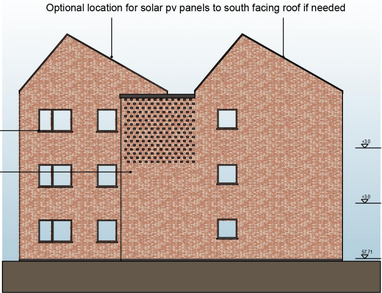
Proposed Rear Elevation (West Facing)
