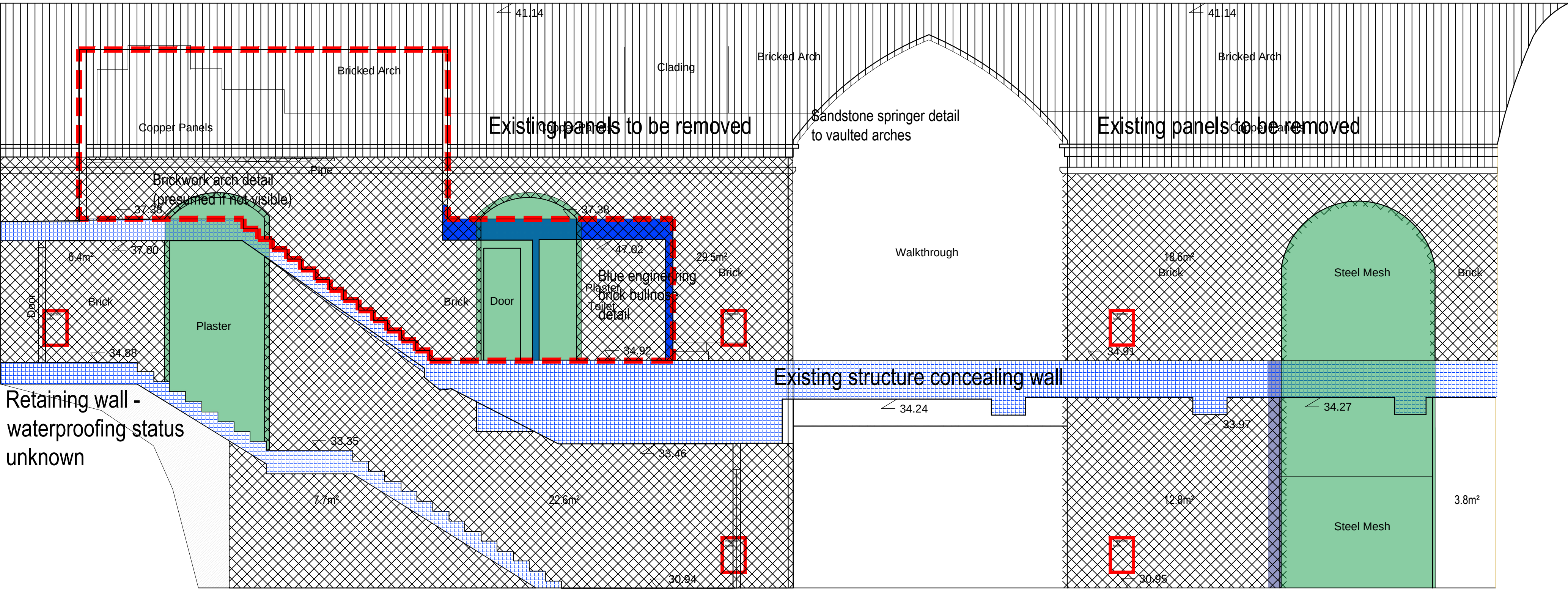
Arch 7 Internal Elevation 2
