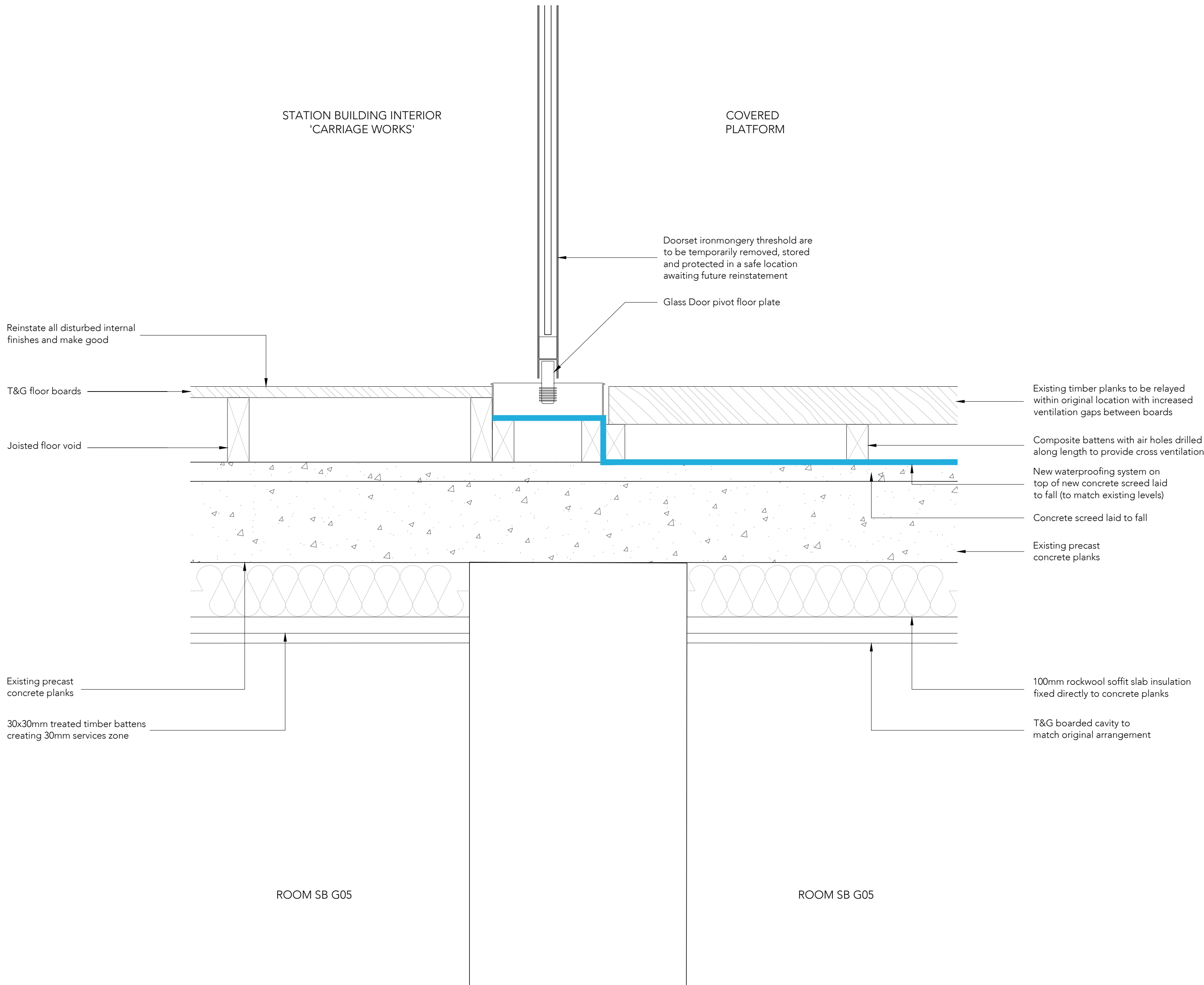
Typical detail through glass door threshold K-K as Proposed Scale 1:5
