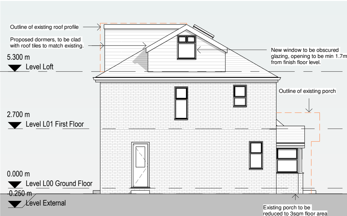
4 Proposed East Elevation 1 : 100
