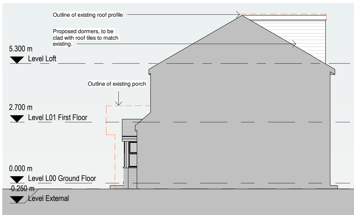
2 Proposed West Elevation 1 : 100
