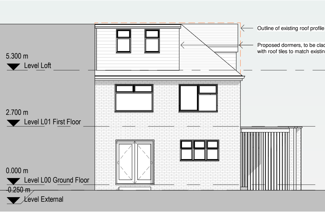
3 Proposed South Elevation 1 : 100
