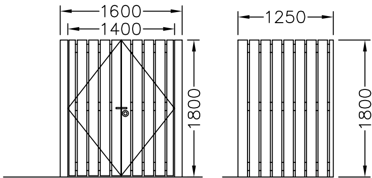
Proposed Bin store Elevation, 1:50
