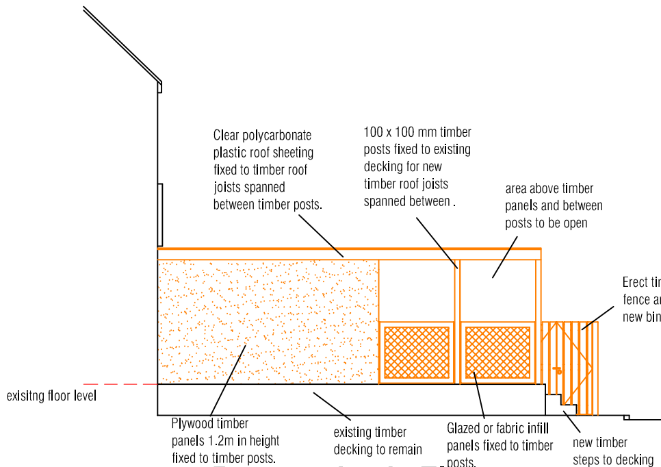
Proposed side Elevation next to No 318, 1:100
