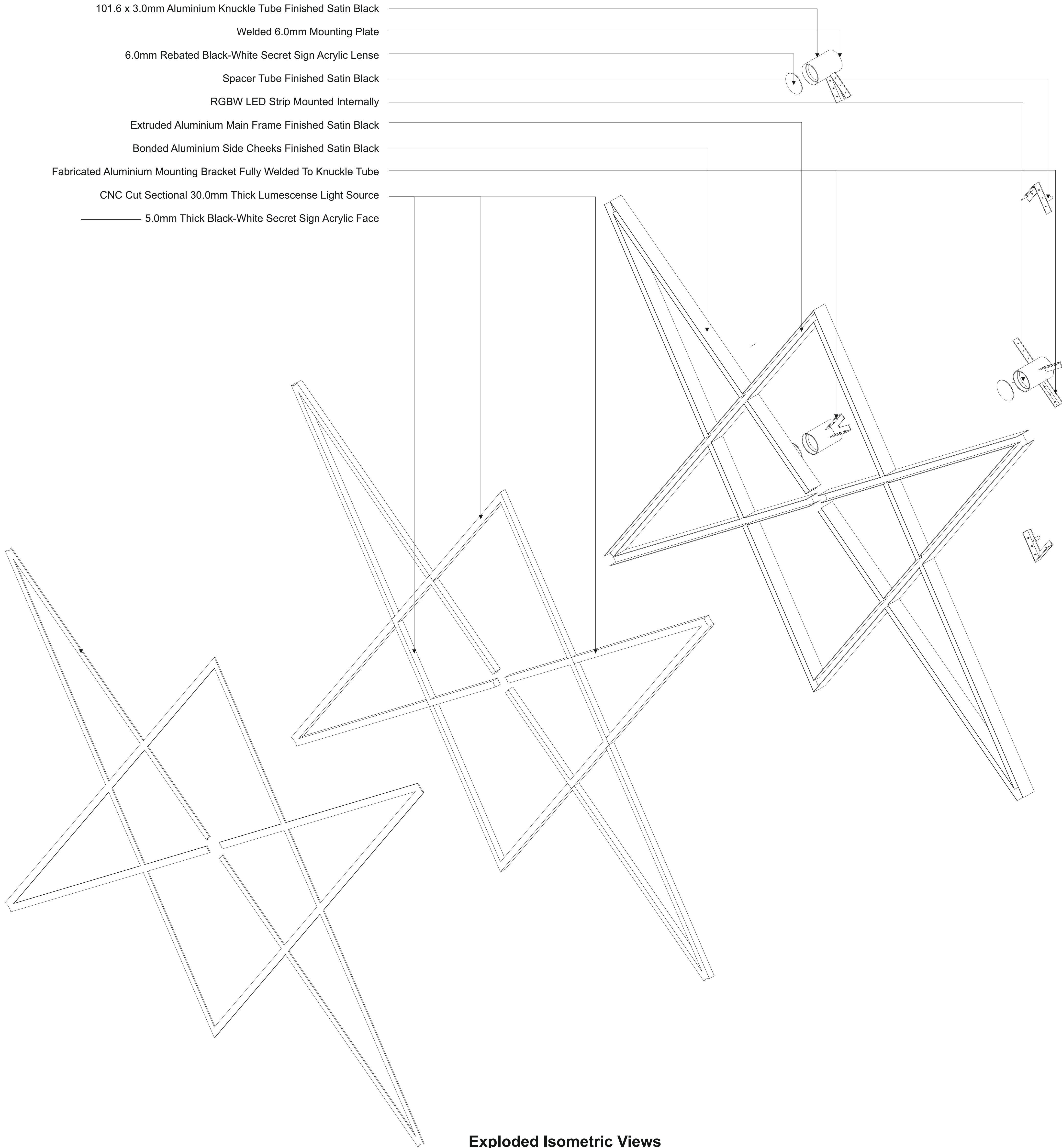
Exploded Isometric Views Scale 1:10 @ A0
