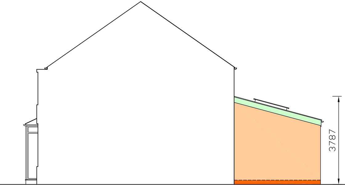
Proposed Sectional / Side Elevation 1:100
