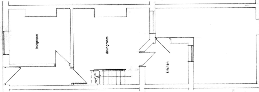
G.F. PLAN (EXISTING)
