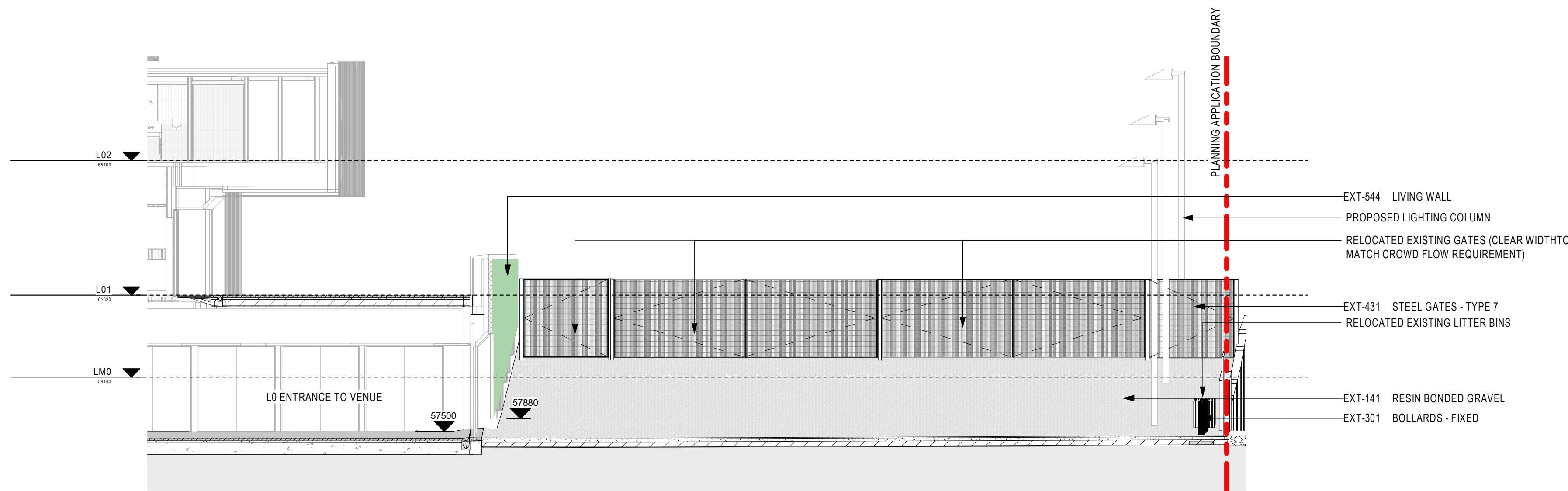
2 SECTION - JOE MERCER WAY ENTRANCE 1:100
