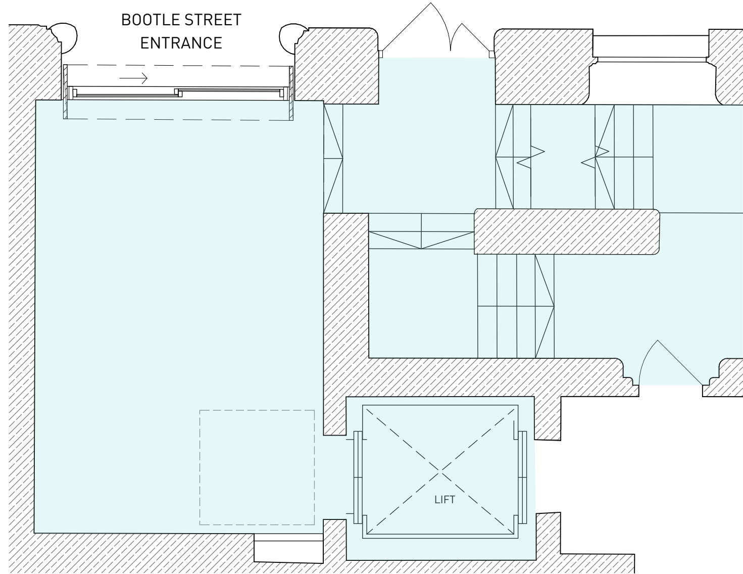
GROUND FLOOR PART PLAN (BOOTLE STREET ENTRANCE)
