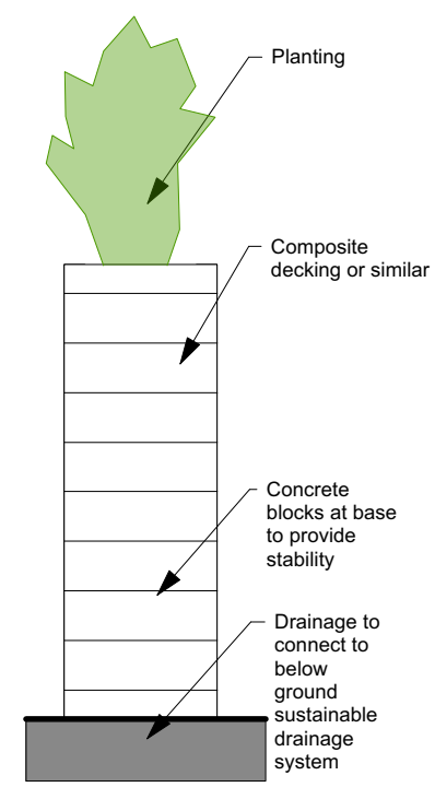
1:20 Planter Detail
