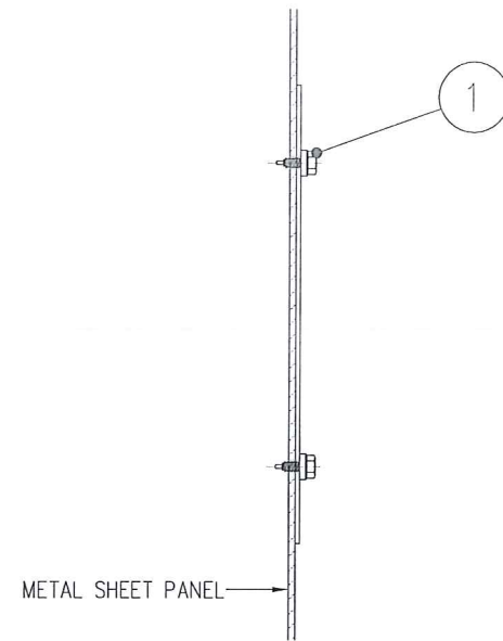
C07a – METAL SHEET PANEL WALL 25MM SCREWS
