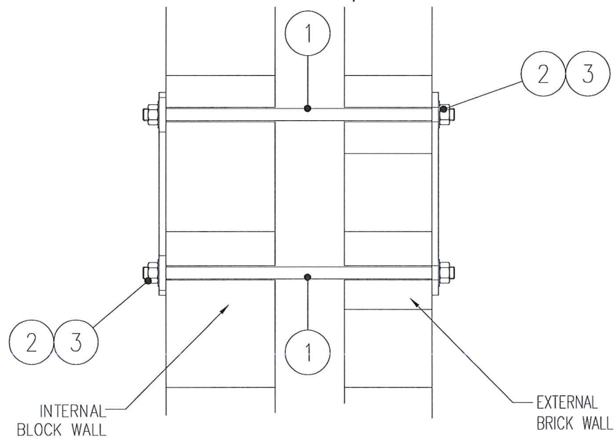
C05c – CAVITY WALL 13–16MM HOLES/SLOTS
