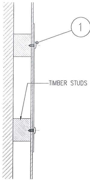
C06a – STUD WALL 12MM SCREWS
