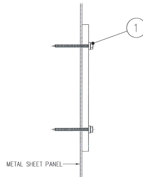
C07d – METAL SHEET PANEL WALL 90MM SCREWS
