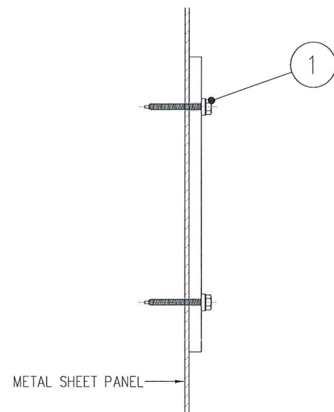
C07c – METAL SHEET PANEL WALL 75MM SCREWS
