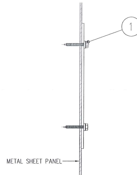
C07b – METAL SHEET PANEL WALL 55MM SCREWS
