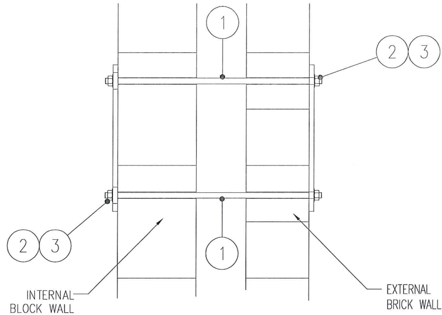
C05a – CAVITY WALL 9/10MM HOLES/SLOTS
