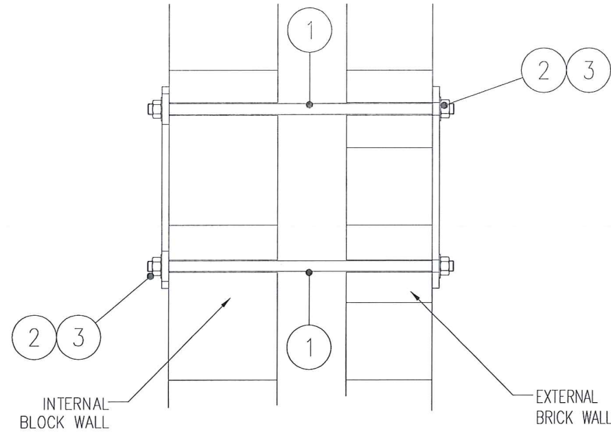
C05b – CAVITY WALL 11/12MM HOLES/SLOTS
