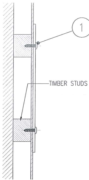
C06b – STUD WALL 25MM SCREWS
