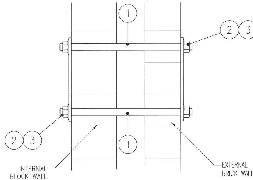
C05d – CAVITY WALL 17–20MM HOLES/SLOTS
