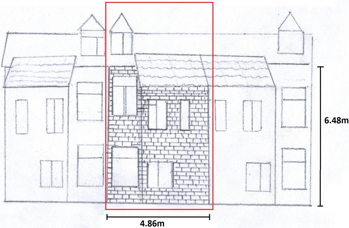
Proposed Back Elevation
