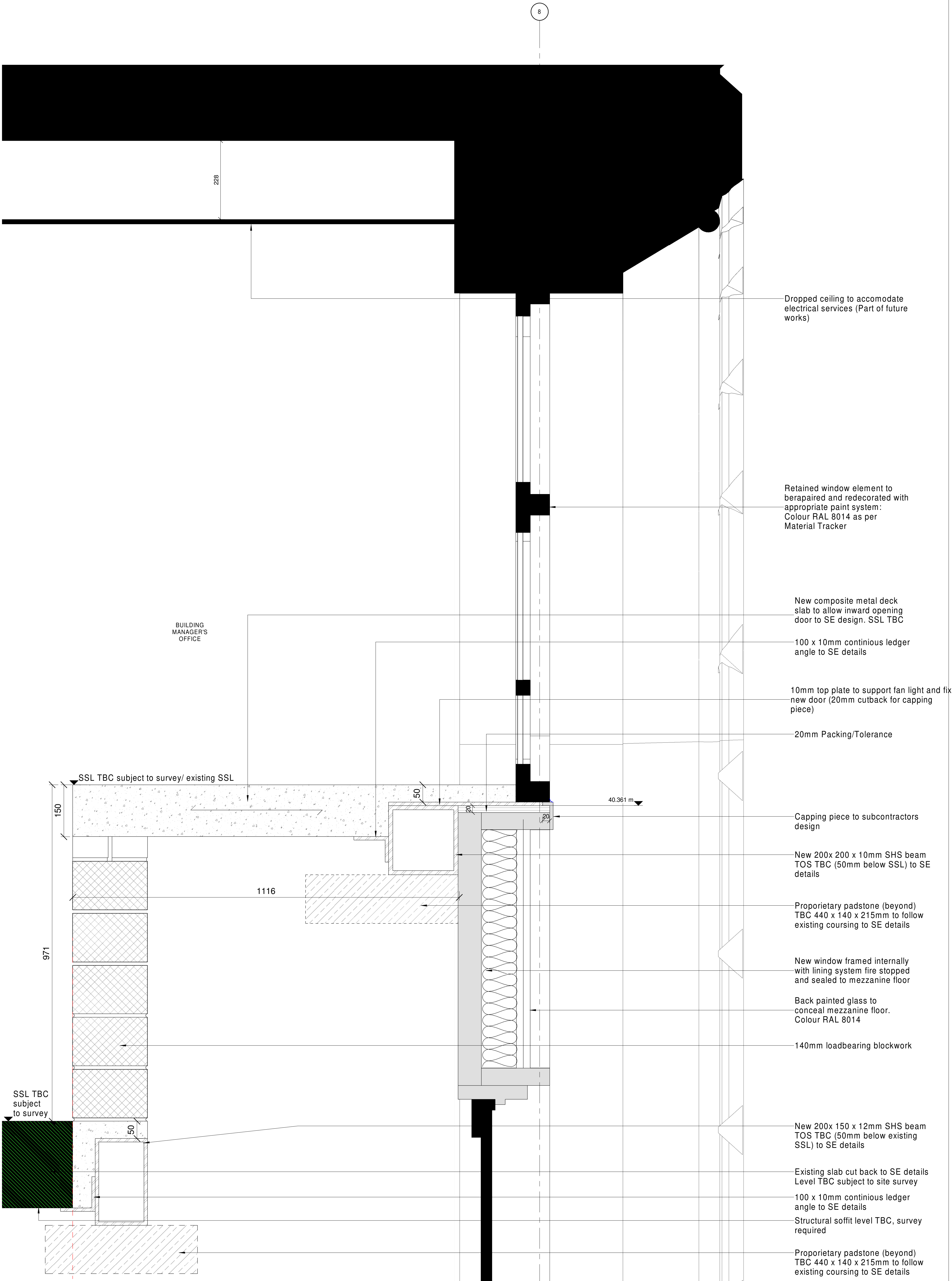
2 External Door Type D - Proposed Section 32651 1:5
