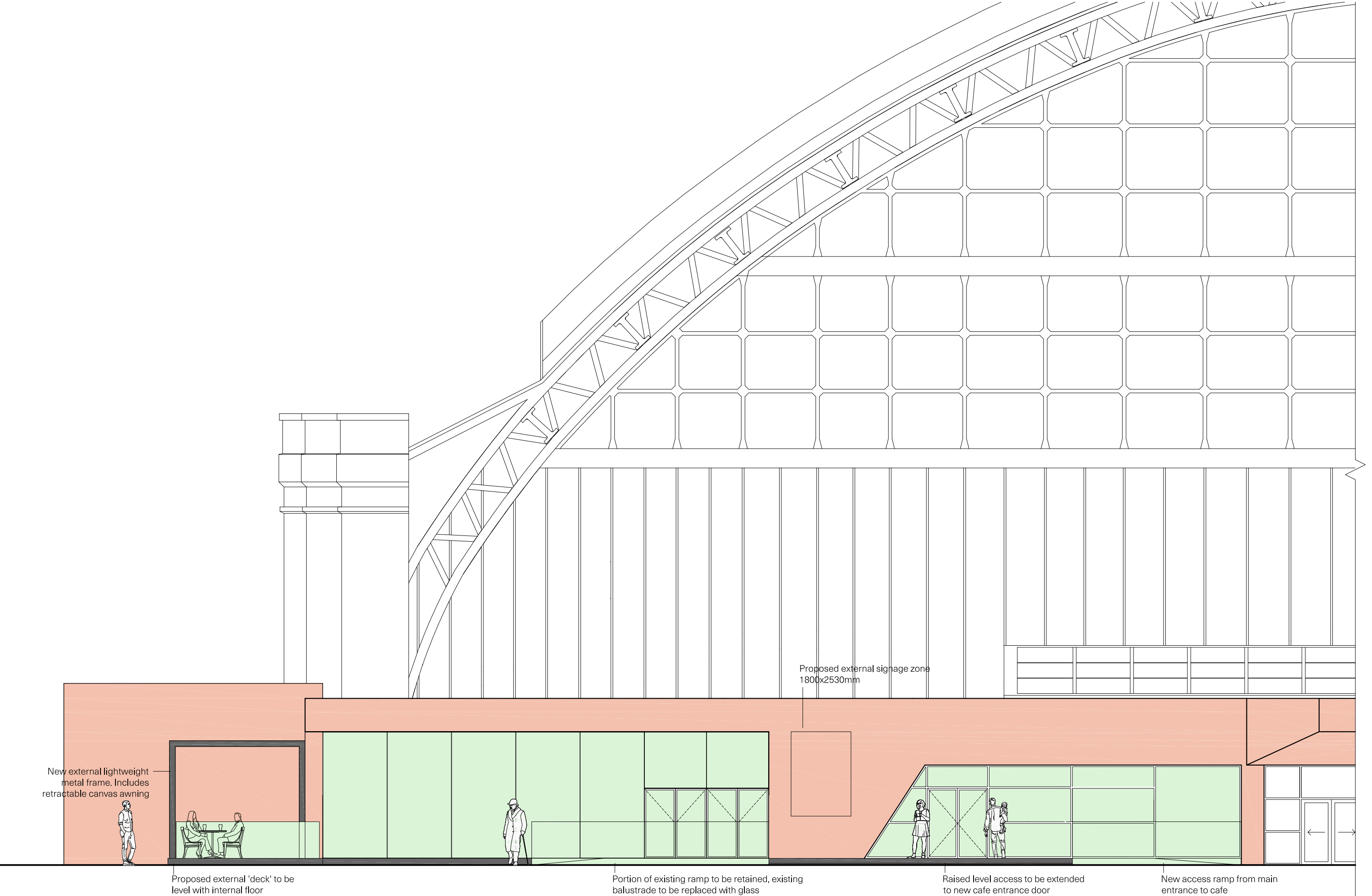
PROPOSED NORTH EAST ELEVATION
