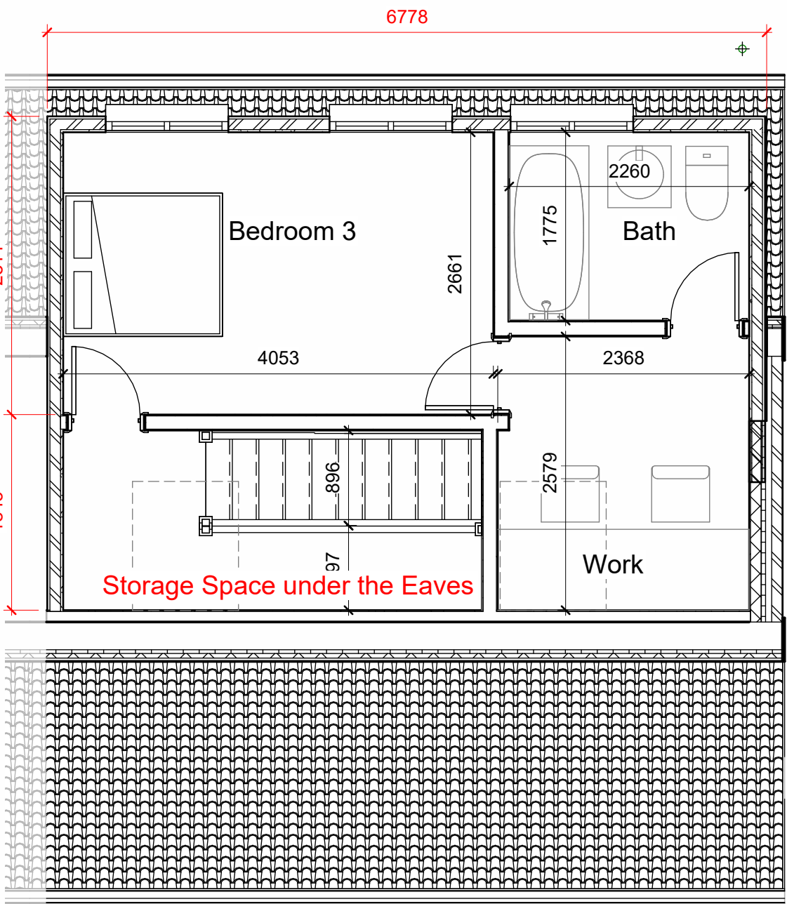
Proposed Loft 1 : 50
