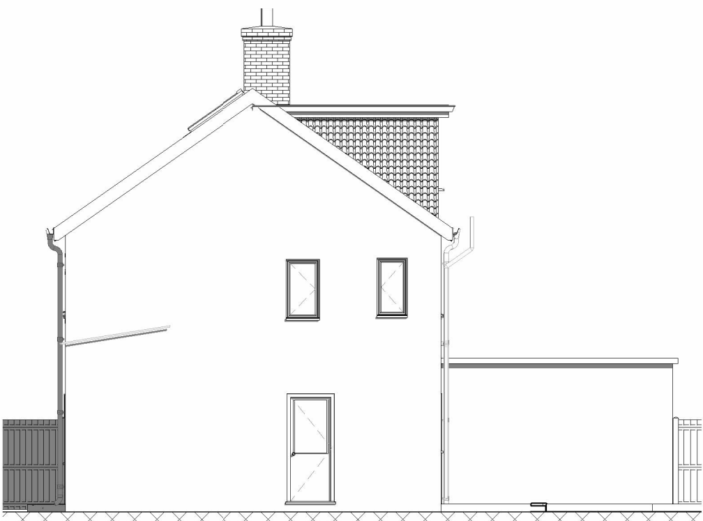
Proposed Side Elevation1 1 : 100
