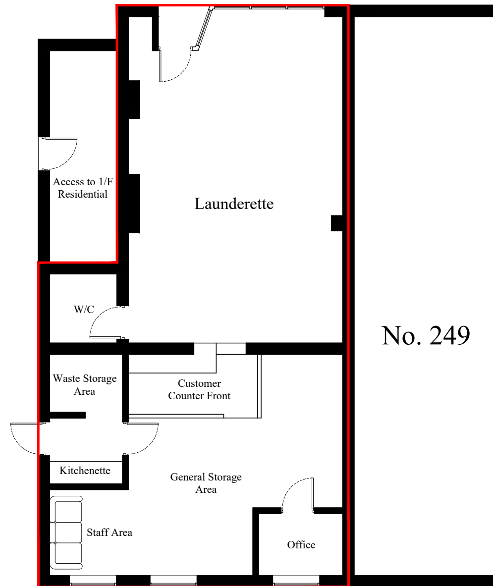
Proposed G/F Plan 1:100
