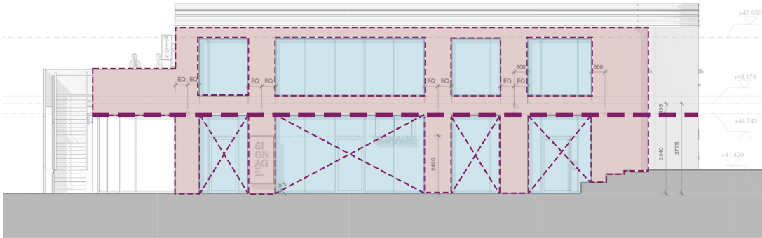
East Elevation | Block C
