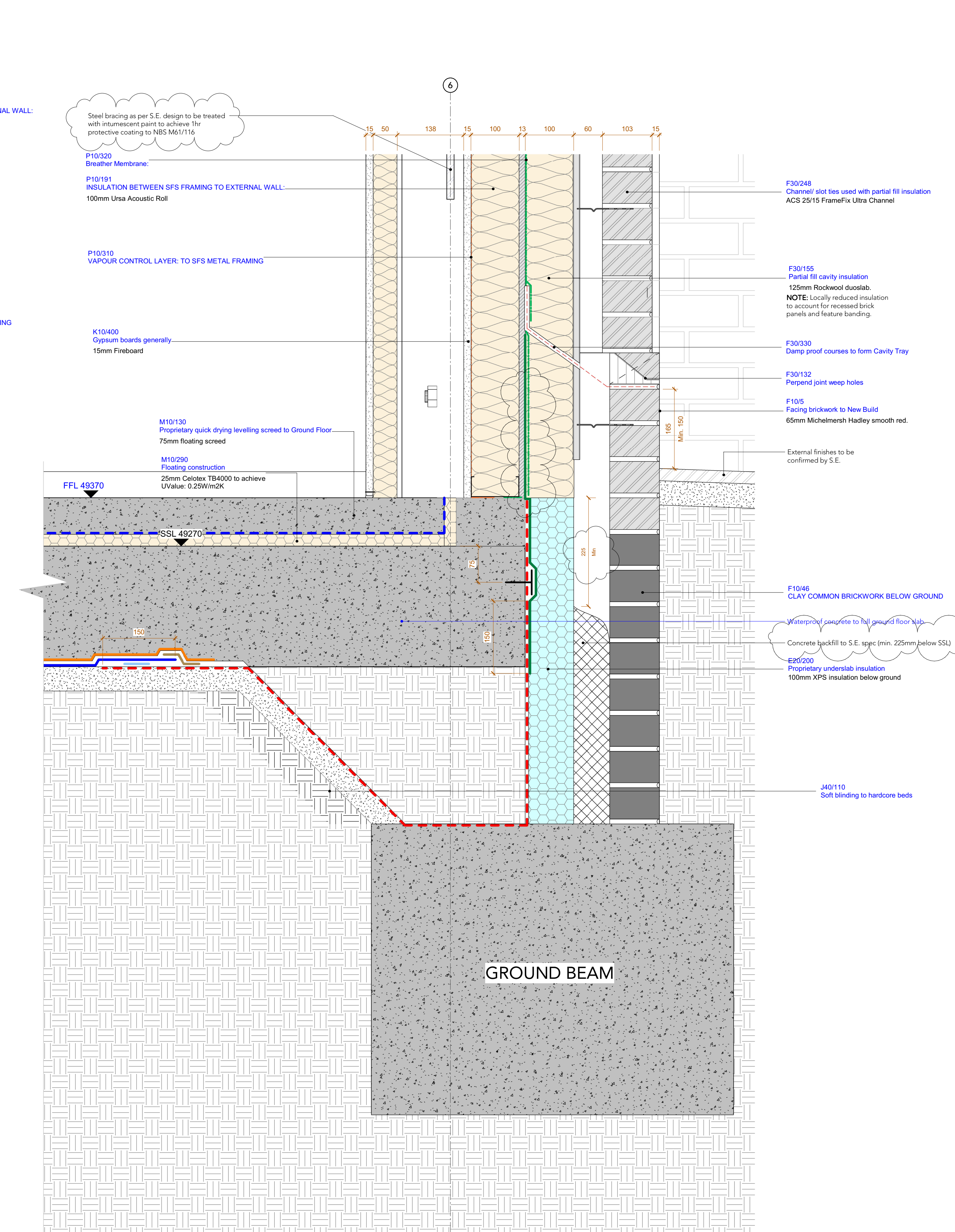
Proposed Ground Floor Section - Stair Core
