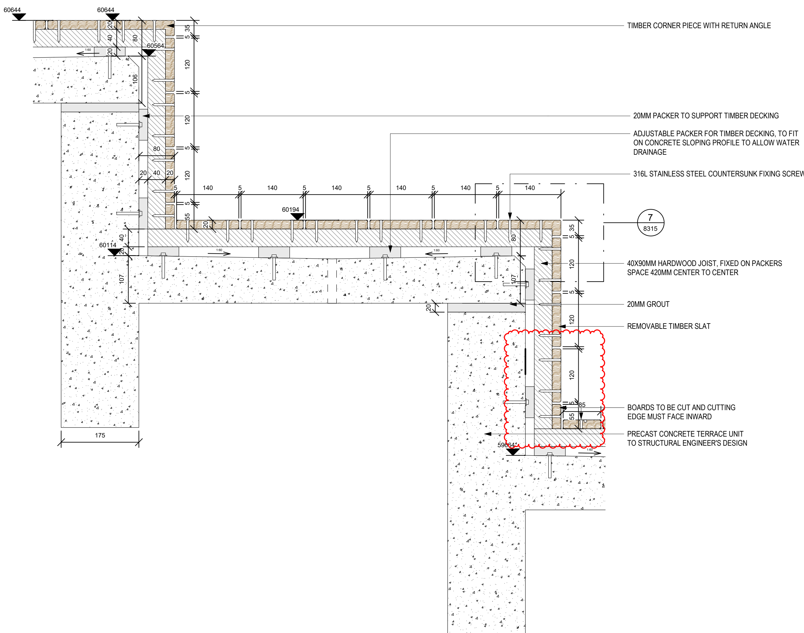
4 TYPICAL SEATING STEP DETAIL
