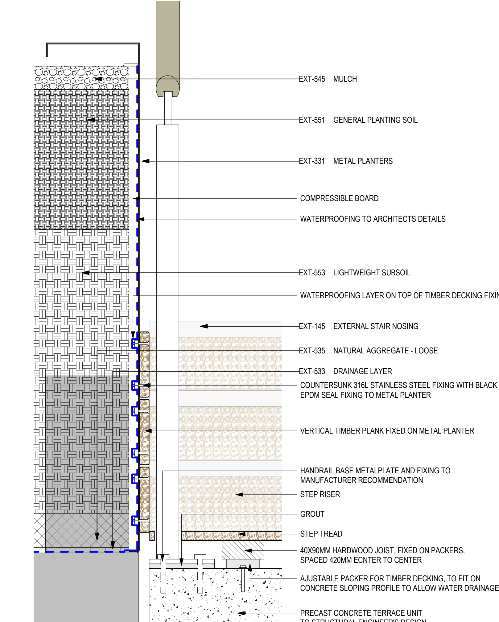
8 TIMBER CLADDING INTERFACE WITH METAL PLANTER
