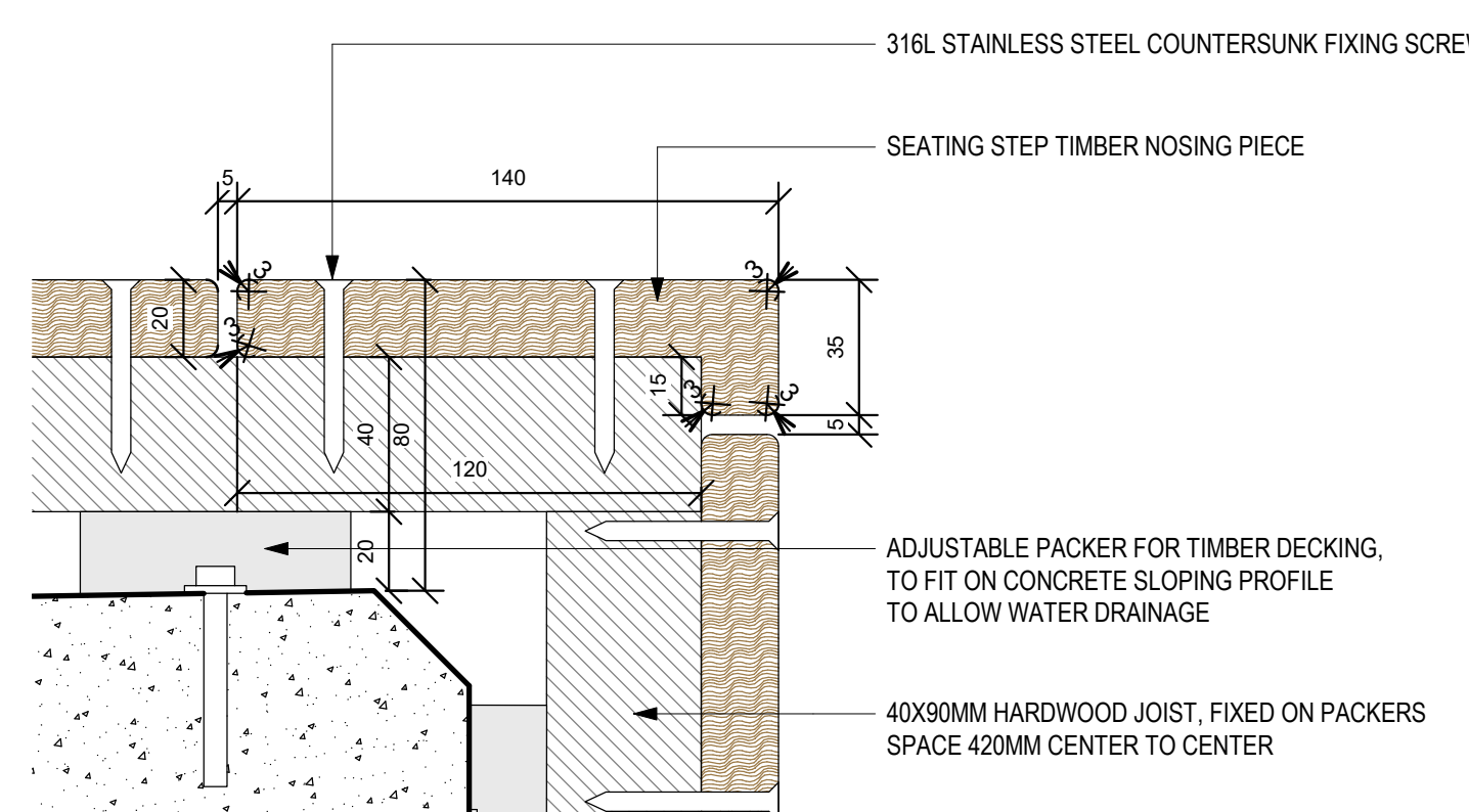
7 STEATING STEP TIMBER NOSING DETAIL
