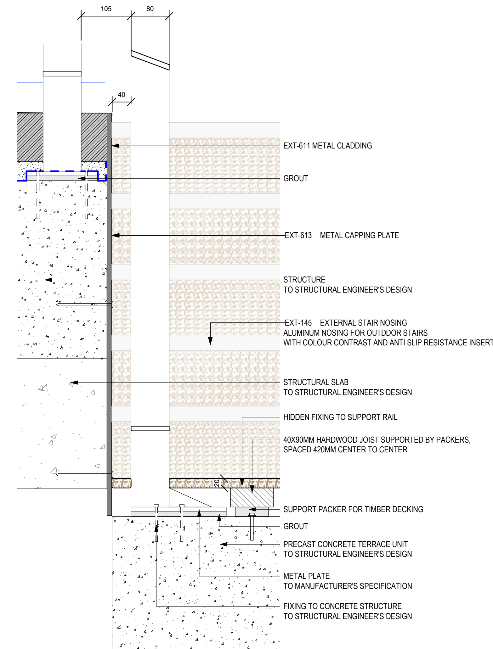
6 TYPICAL METAL CLADDING DETAIL
