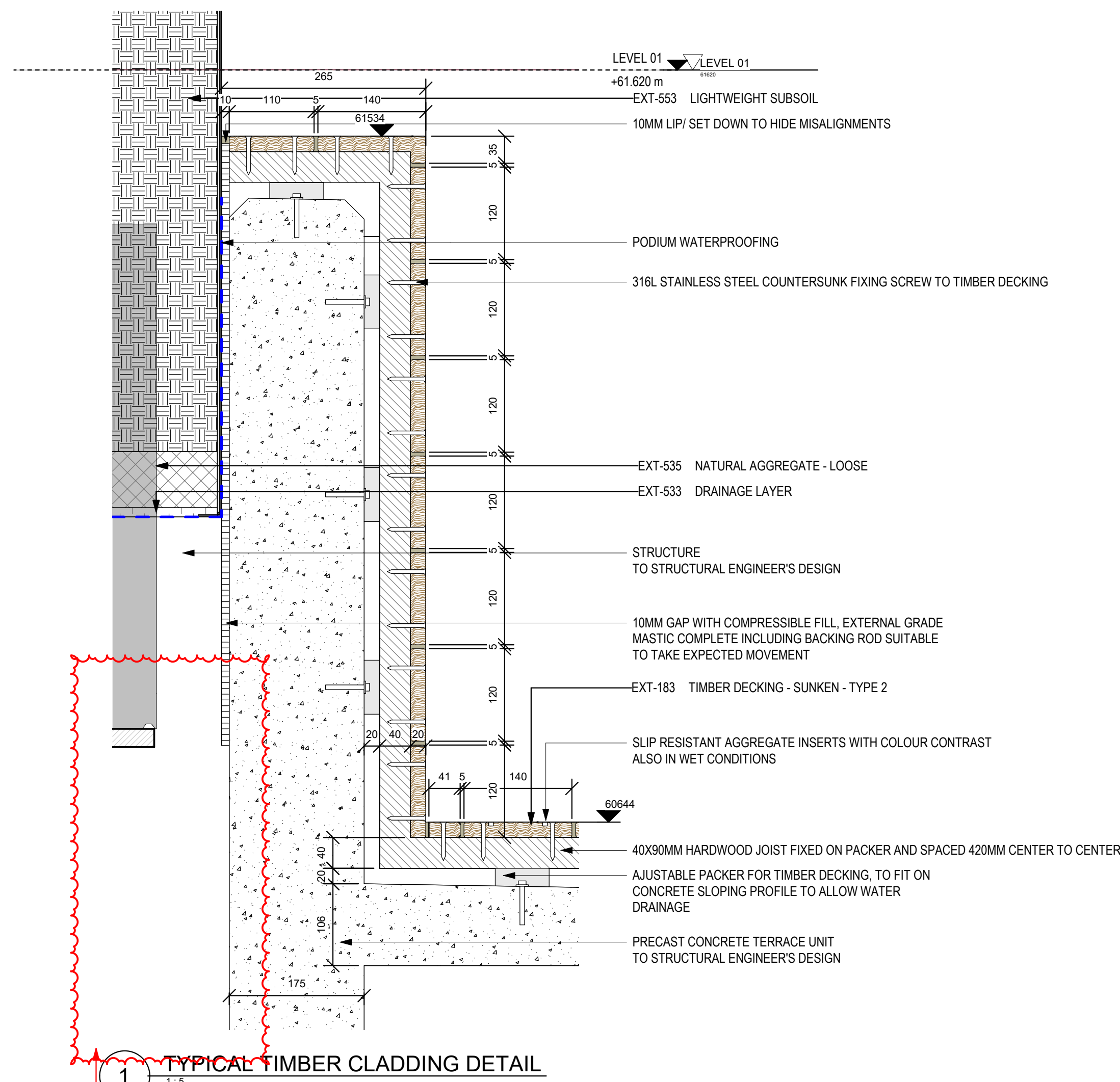
1 TYPICAL TIMBER CLADDING DETAIL
