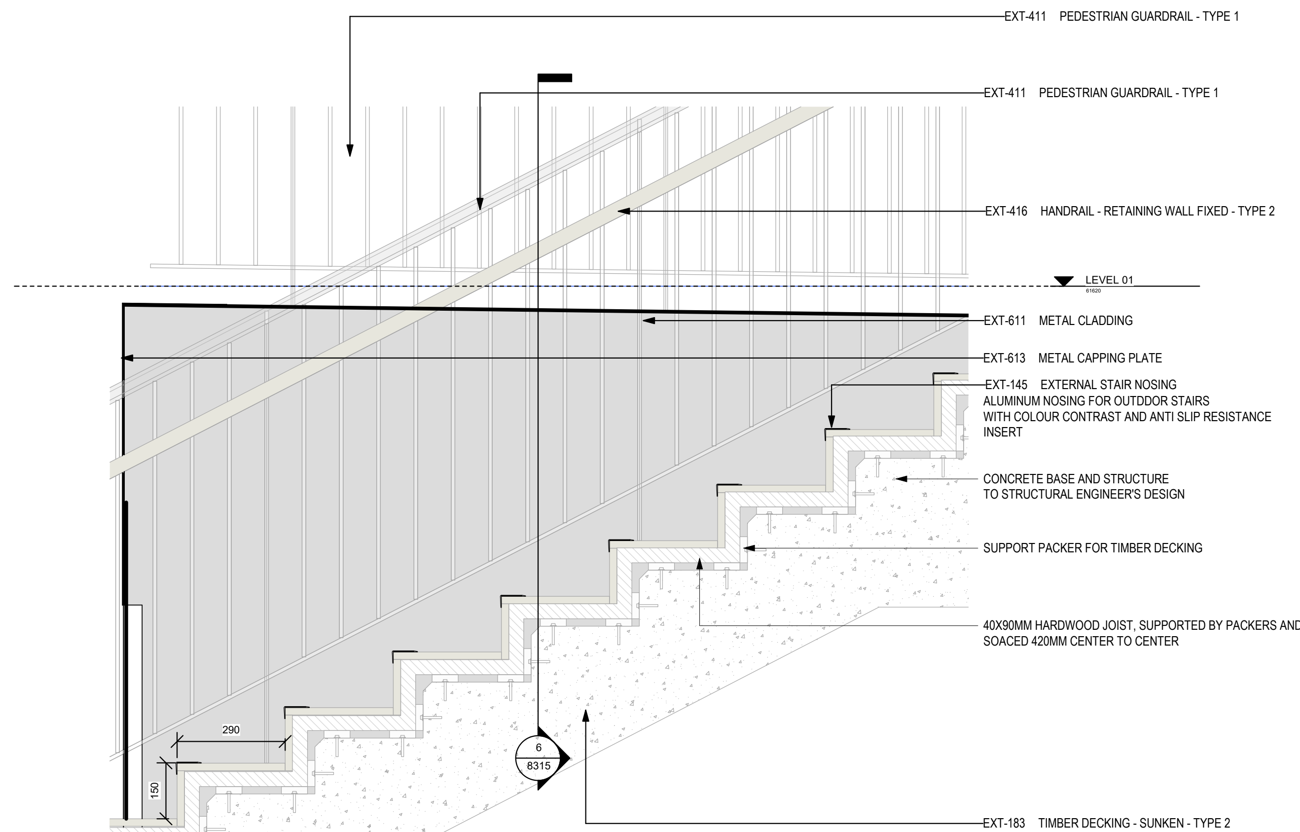
5 METAL CLADDING NEXT TO TIMBER STAIRS ELEVATION
