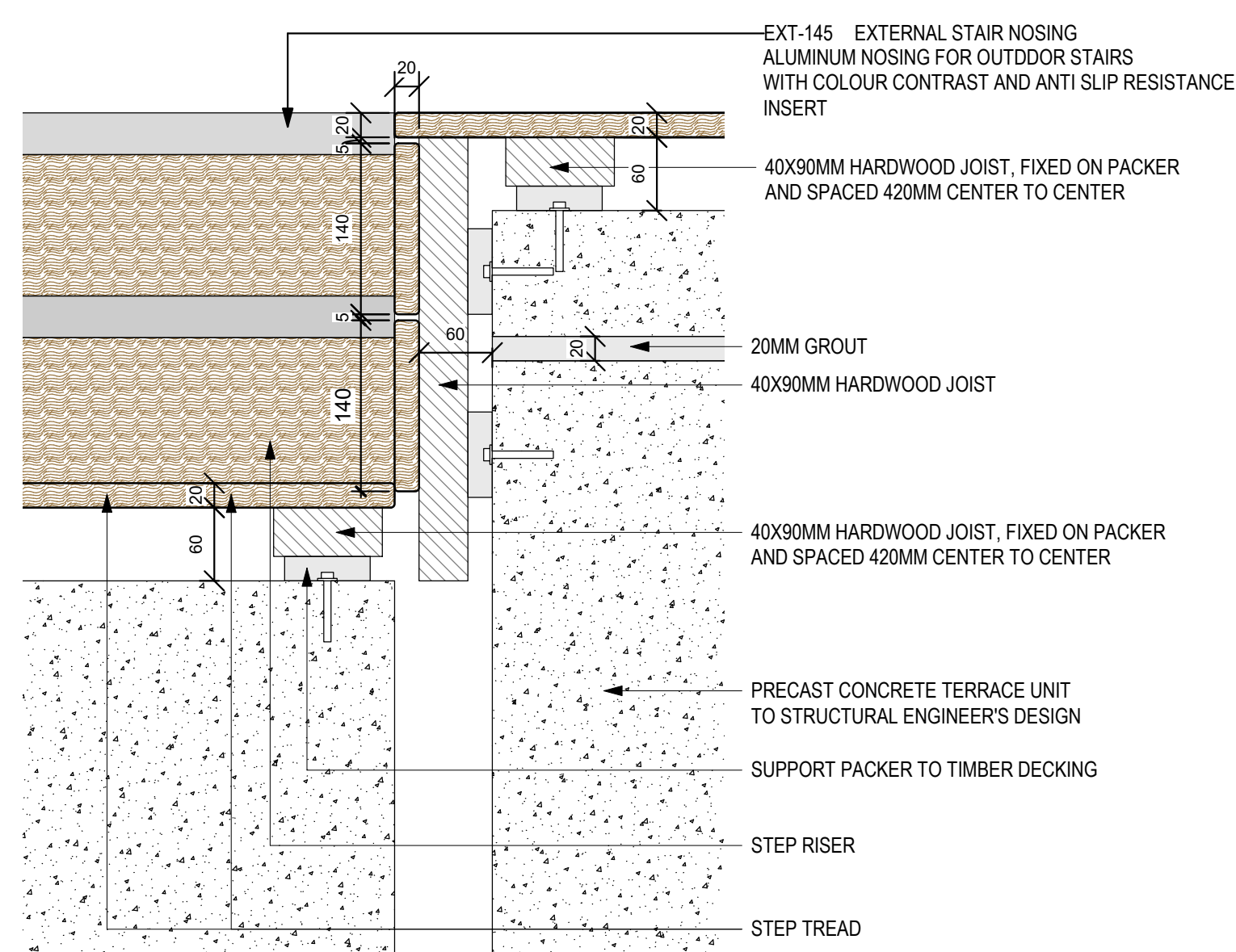
2 TIMBER STAIRS SIDE CLADDING DETAIL
