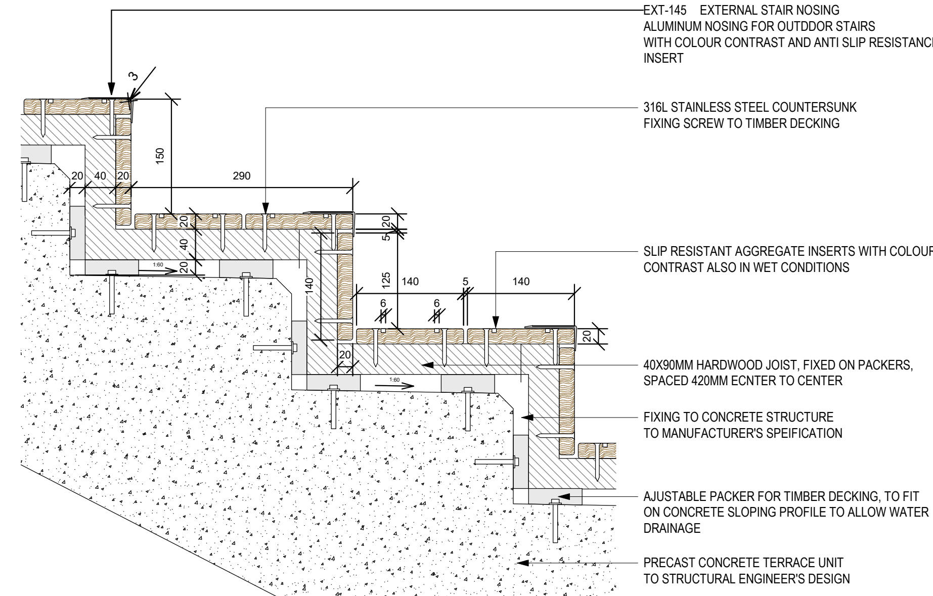
3 TYPICAL TIMBER STEP DETAIL
