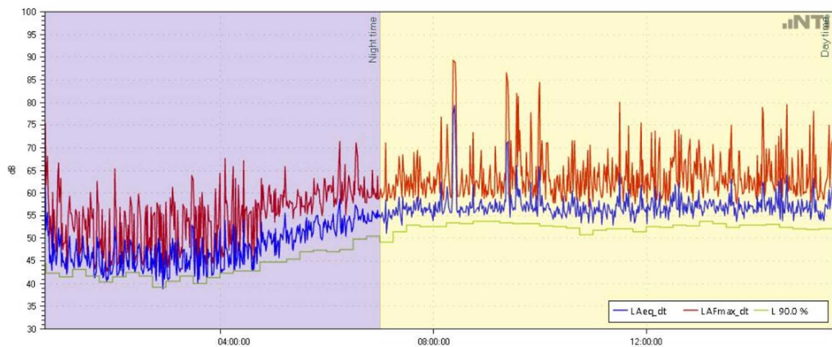
Figure 4 Time history
