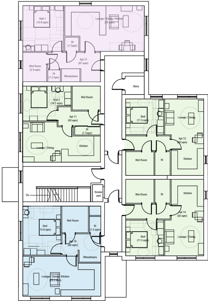
Second Floor - Internal Floor Area = 363 sqm 1 No. M4 (3) 1b2p Apt @ 60 sqm 1 No. M4 (3) 1b2p Apt @ 67 sqm 3 No. M4 (2) 1b2p Apts @ 50 sqm
