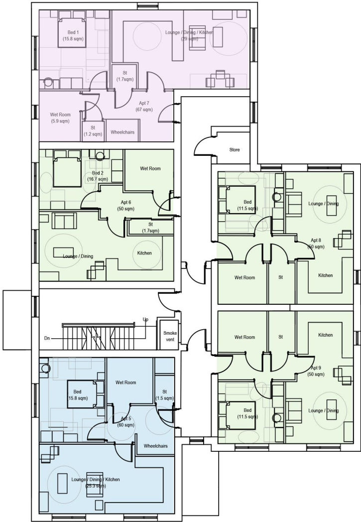
First Floor - Internal Floor Area = 363 sqm 1 No. M4 (3) 1b2p Apt @ 60 sqm 1 No. M4 (3) 1b2p Apt @ 67 sqm 3 No. M4 (2) 1b2p Apts @ 50 sqm
