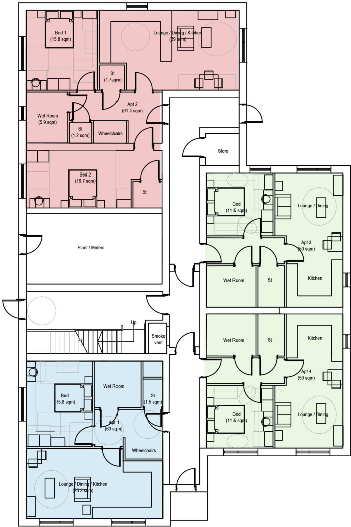
Ground Floor - Internal Floor Area = 368 sqm 1 No. M4 (3) 1b2p Apt @ 60 sqm 1 No. M4 (3) 2b4p Apt @ 91.4 sqm 2 No. M4 (2) 1b2p Apts @ 50 sqm
