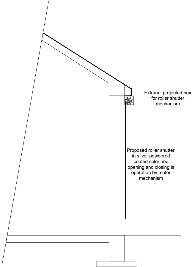
PROPOSED SECTION AA (SCALE 1:50)
