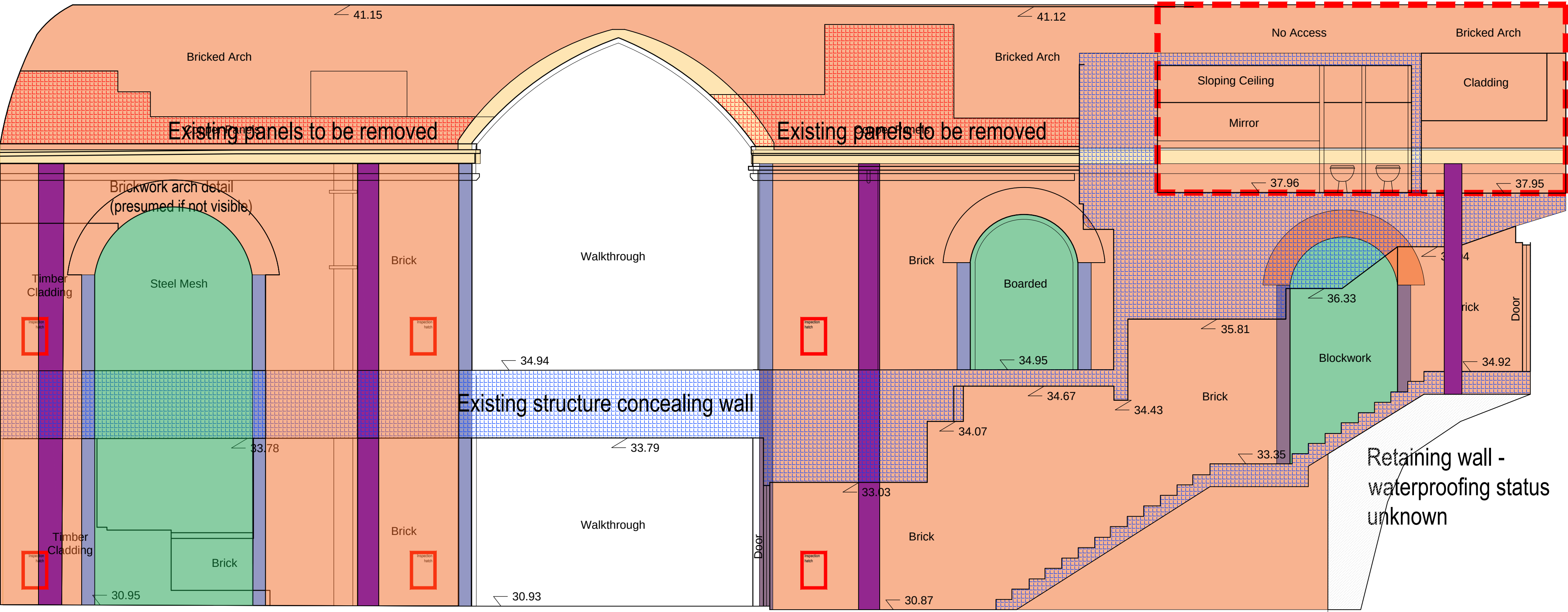
Arch 8 Internal Elevation 1
