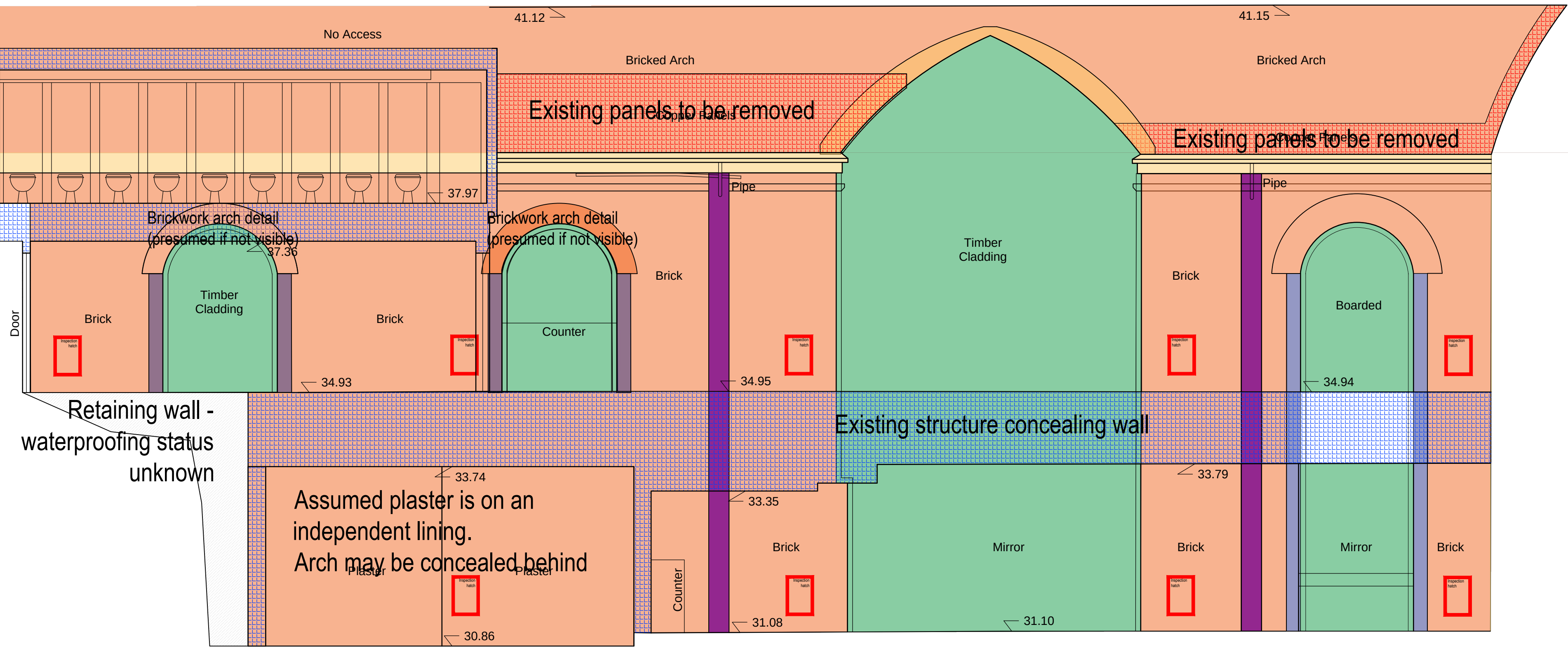
Arch 8 Internal Elevation 2
