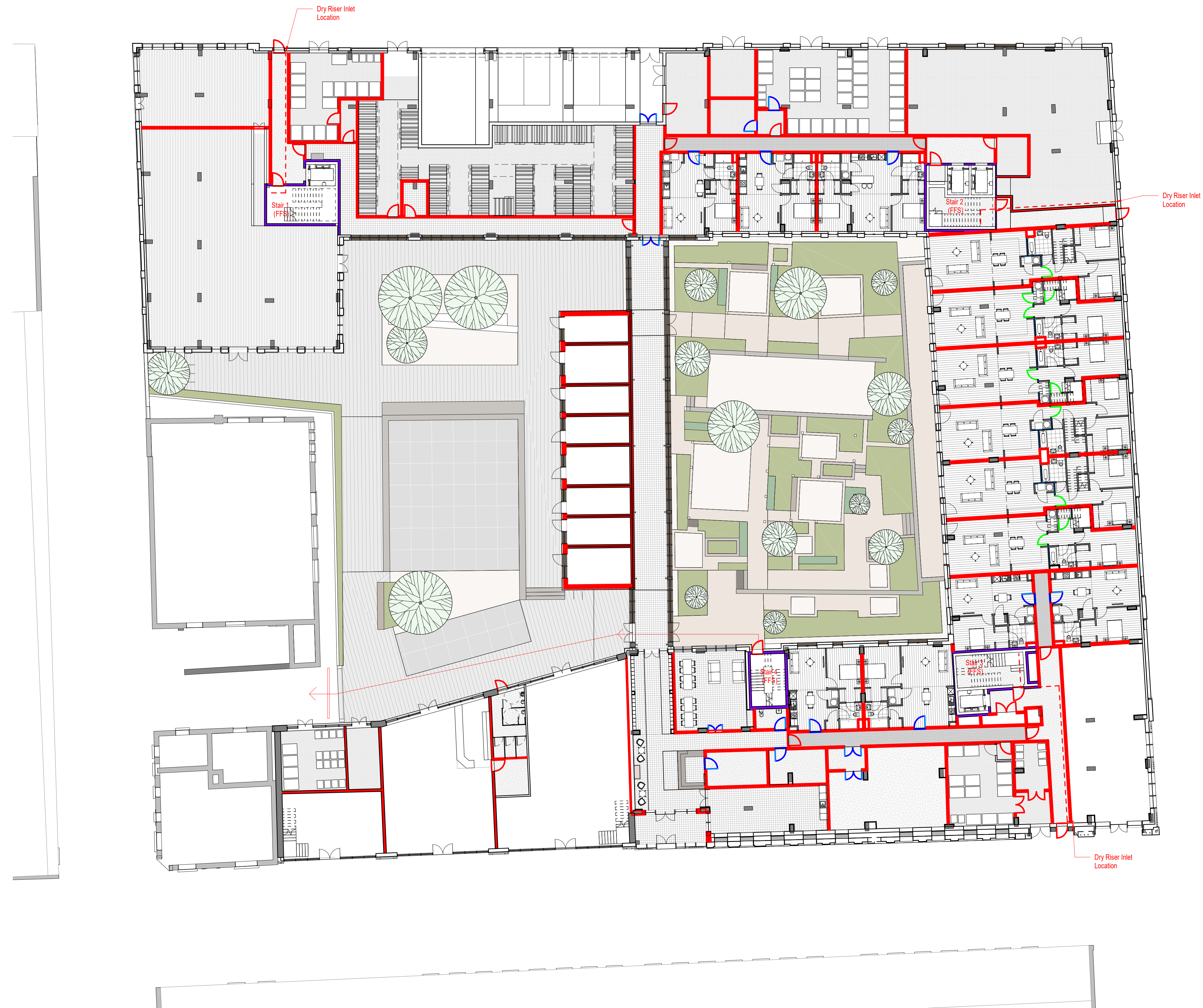
FIRE PLAN LEVEL 00 SCALE: 1 : 200
