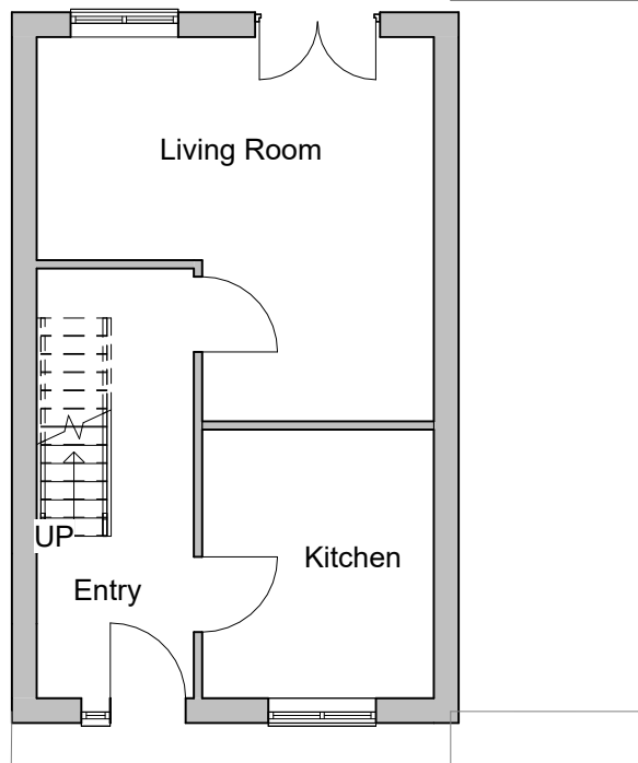
1 Ground Floor 1 : 100
