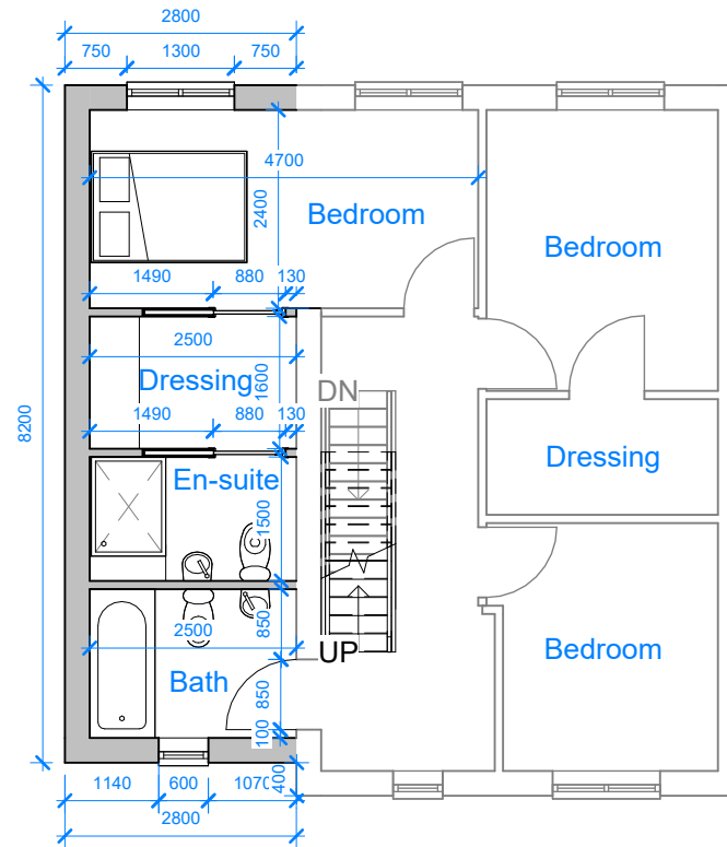
2 First Floor 1 : 100
