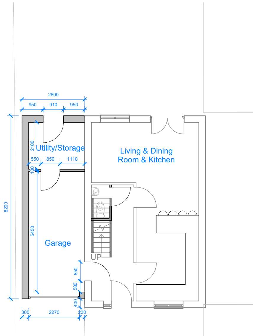
1 Ground Floor 1 : 100
