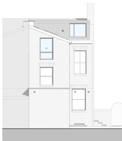
PROPOSED ELEVATIONS - NORTH-WEST
