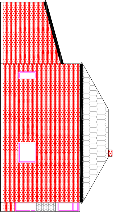
Existing Side elevation (Neighbour 18 side)
