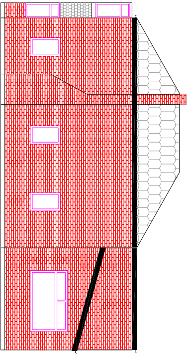
Proposed Side elevation (Neighbour 14 side)
