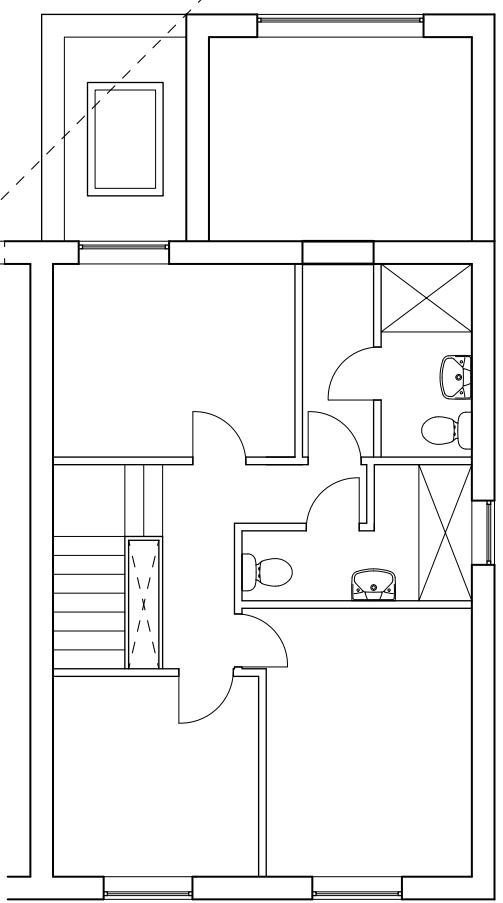
FIRST FLOOR SCALE 1:100 PROPOSED - P004
