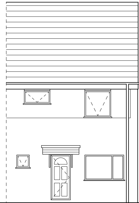
SOUTH EAST ELEVATION SCALE 1:100 PROPOSED - P006
