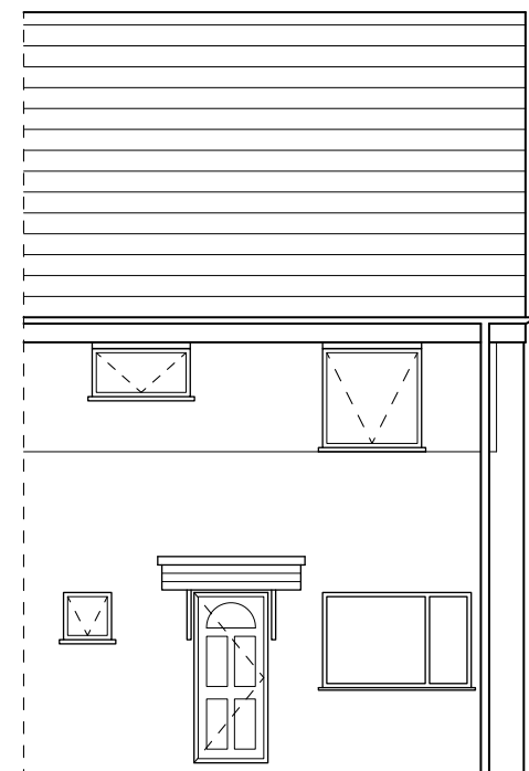
SOUTH EAST ELEVATION SCALE 1:100 EXISTING - E005
