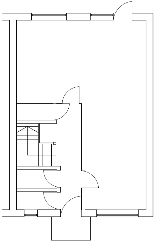
GROUND FLOOR SCALE 1:100 EXISTING - E003
