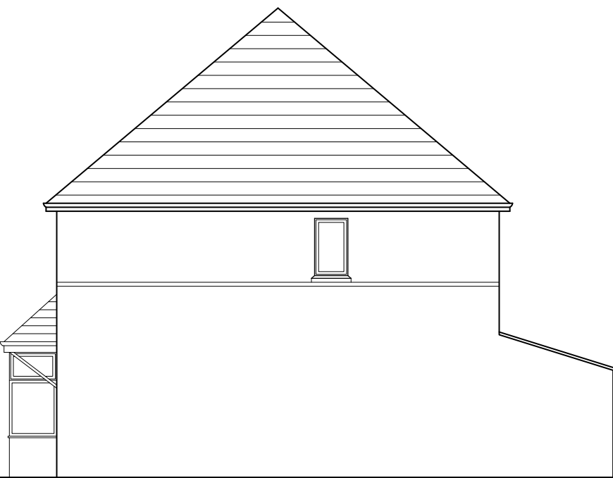
EAST ELEVATION SCALE 1:100 EXISTING - E006
