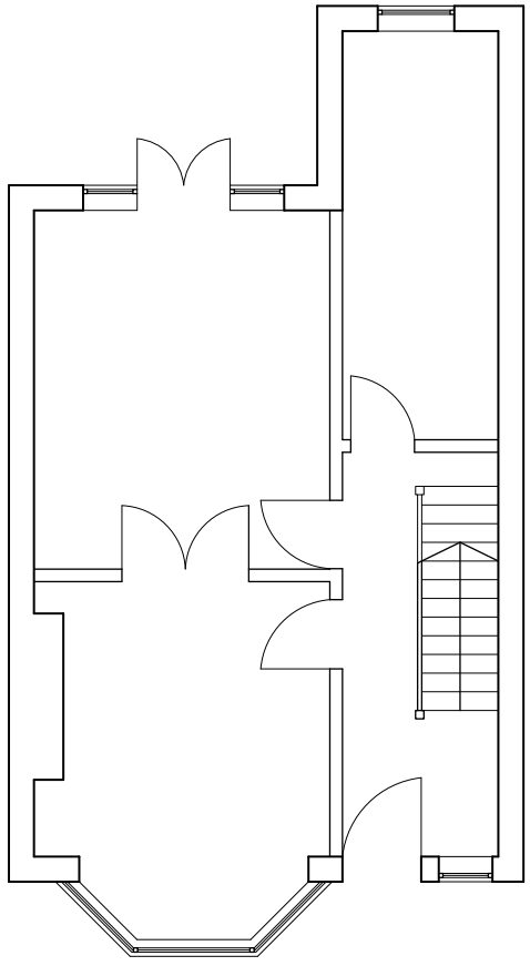
GROUND FLOOR SCALE 1:100 EXISTING - E003
