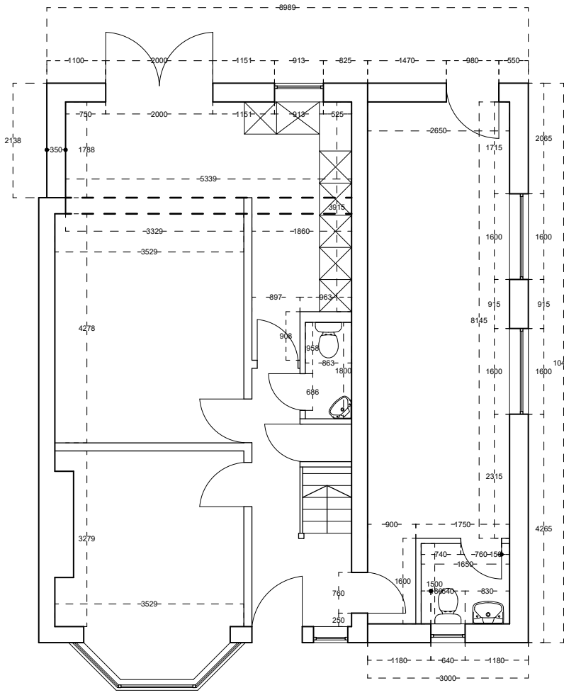
GROUND FLOOR SCALE 1:100 PROPOSED - P003
