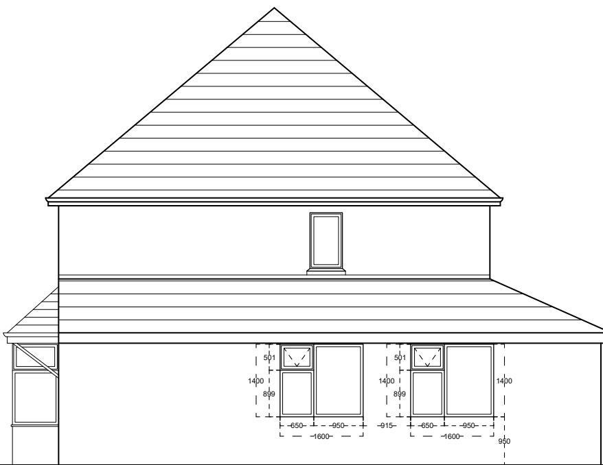
EAST ELEVATION SCALE 1:100 PROPOSED - P007
