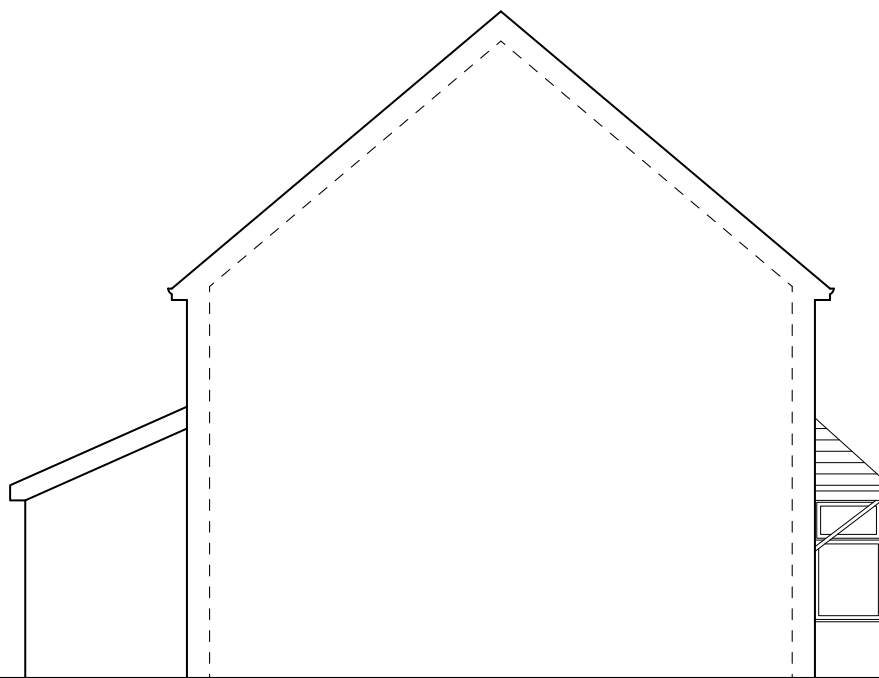
WEST ELEVATION SCALE 1:100 PROPOSED - P009
