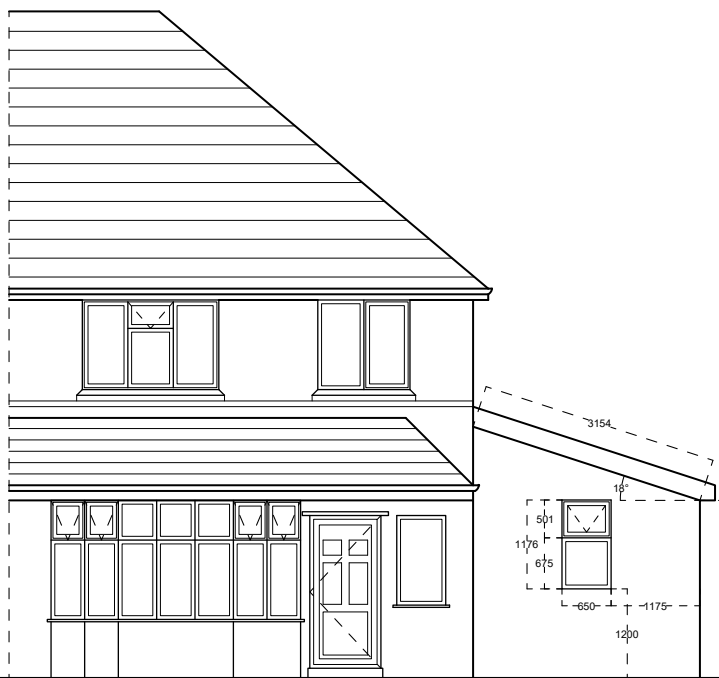
SOUTH ELEVATION SCALE 1:100 PROPOSED - P006
