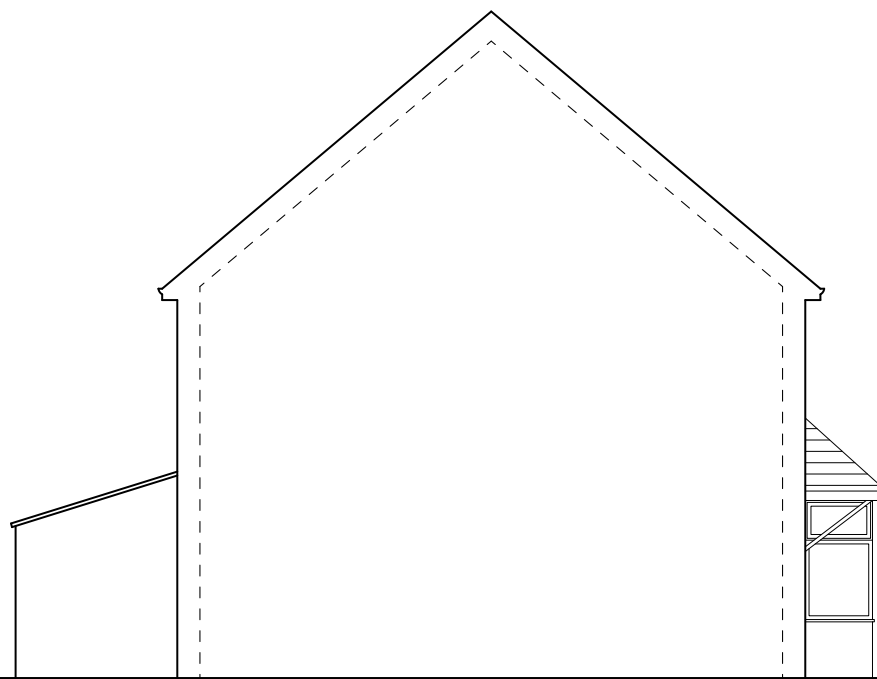
WEST ELEVATION SCALE 1:100 EXISTING - E008
