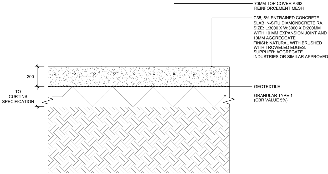
2A 00600 ST02: REINFORCED IN-SITU DIAMONDCRETE RA SECTION
