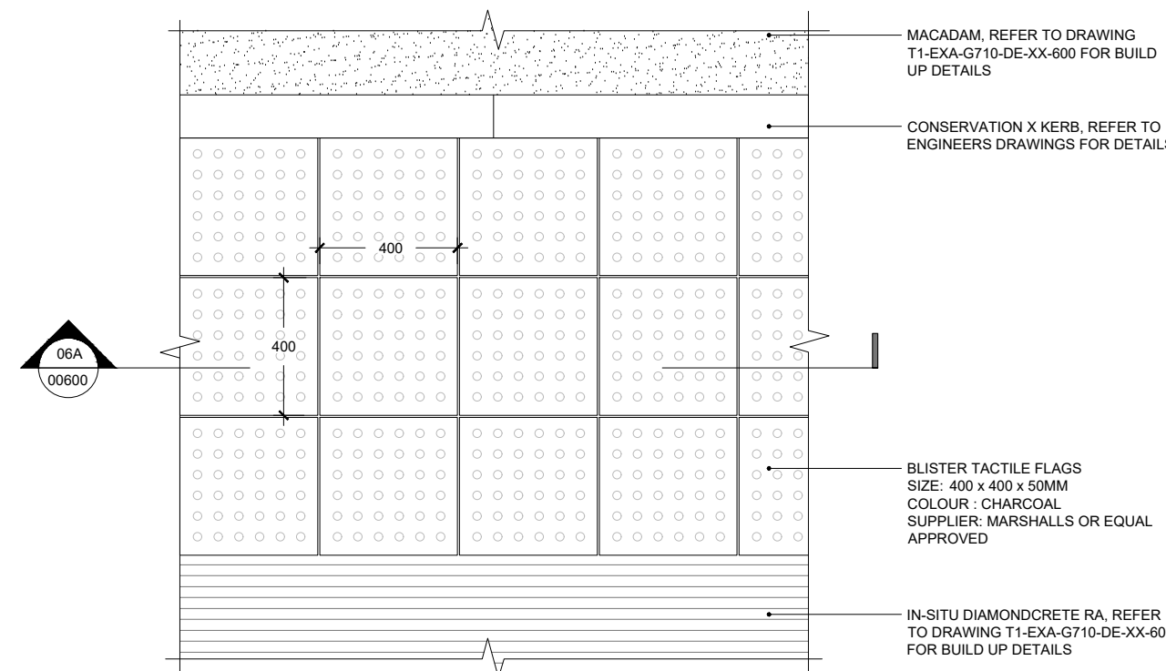
06B 00600 ST06: BLISTER CONCRETE PAVING PLAN
