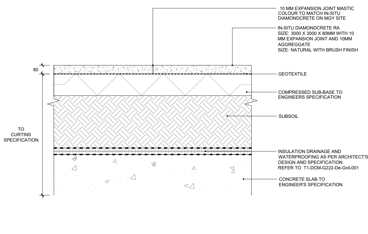
01C 00600 ST01: IN-SITU DIAMONDCRETE RA ABOVE BASEMENT SECTION
