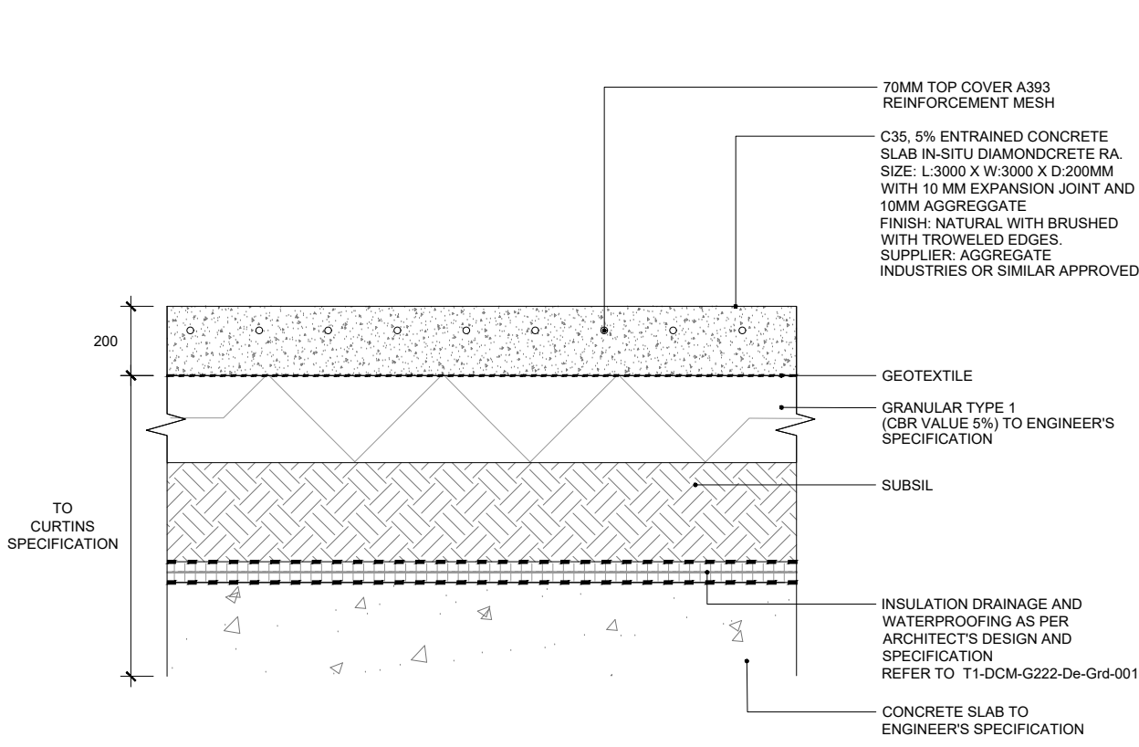
02C 00600 ST02: REINFORCED IN-SITU DIAMONDCRETE RA ABOVE BASEMENT SECTION
