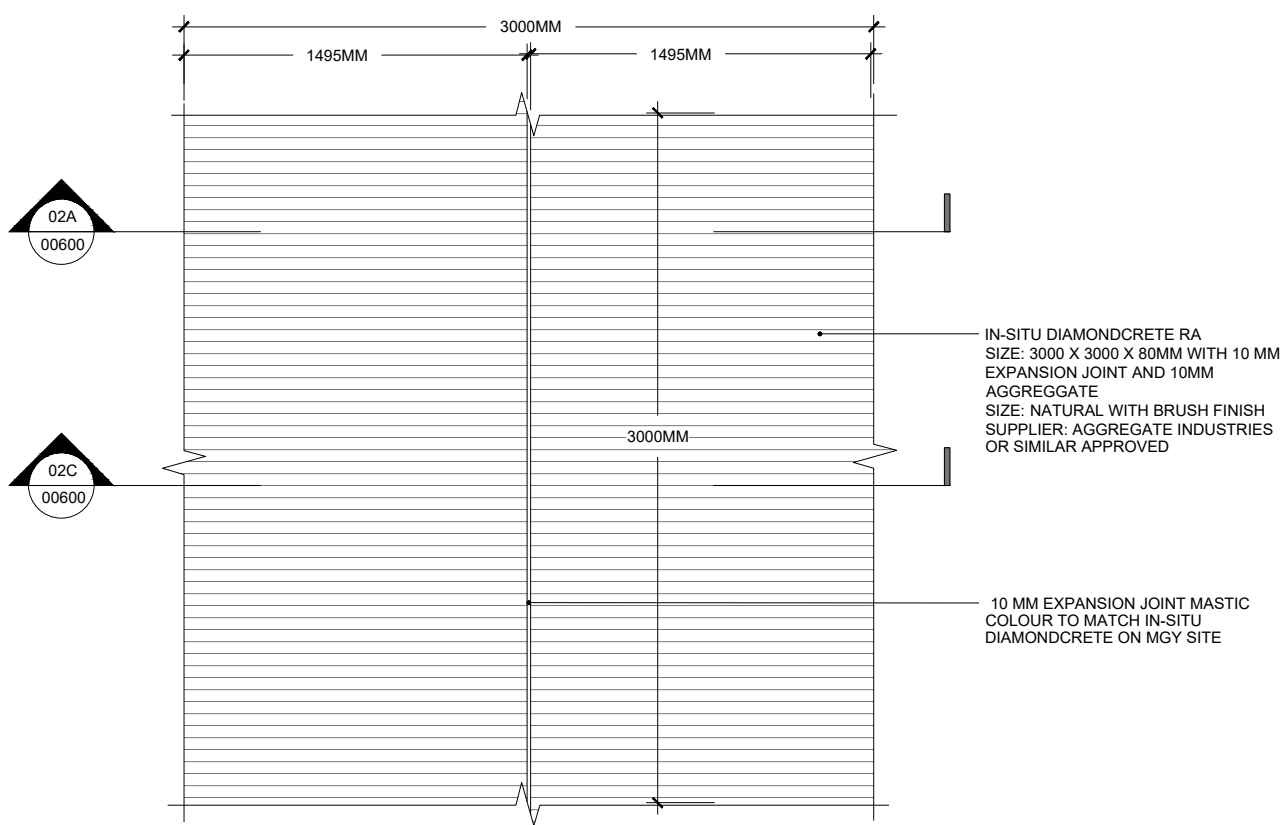
02B 00600 ST02: REINFORCED IN-SITU DIAMONDCRETE RA PLAN
