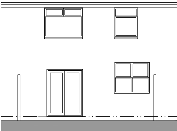
South West Facing Rear Elevation
