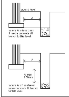
Diagram 8 Pipe runs near buildings
