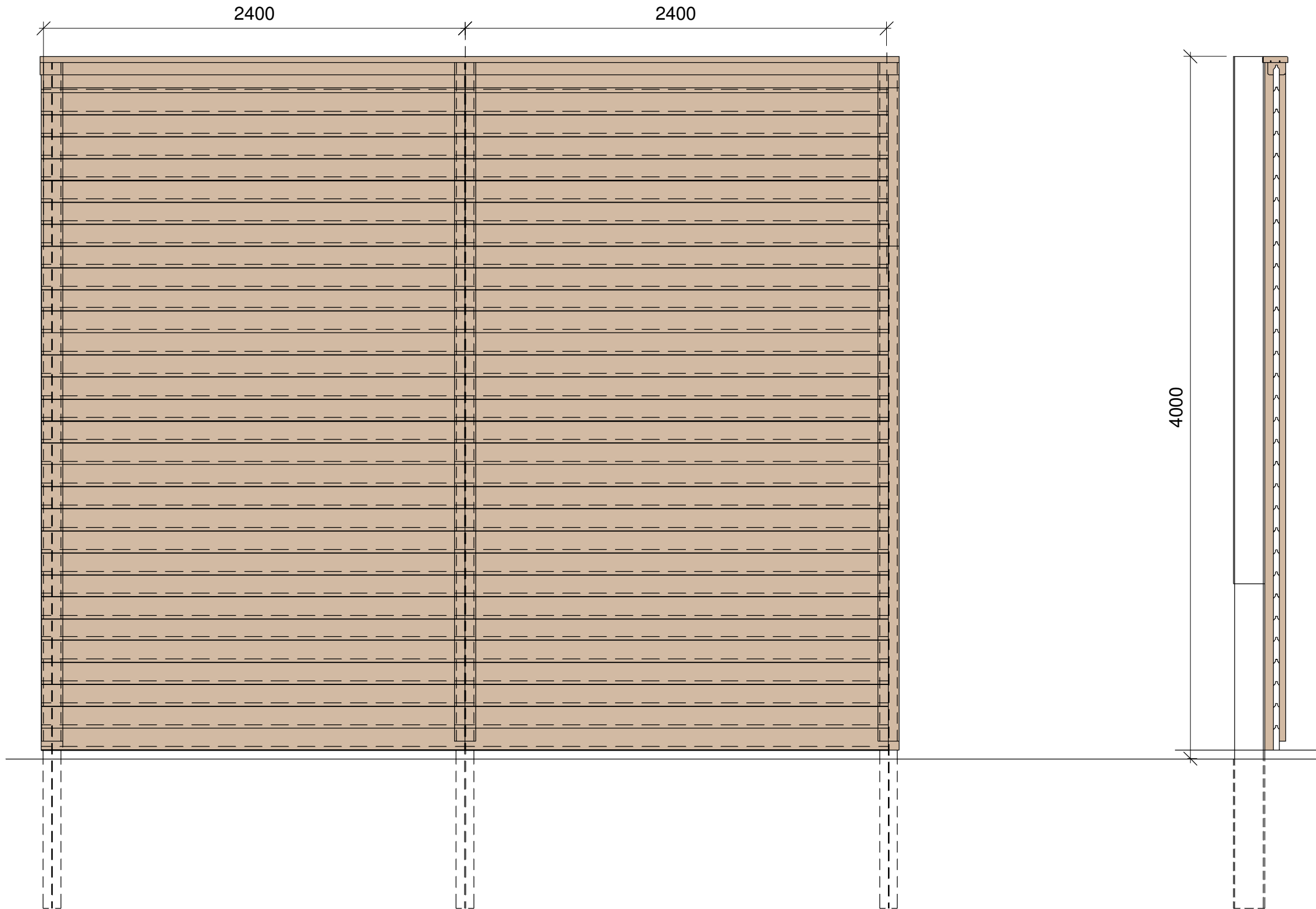
Acoustic Fence 1 : 25
