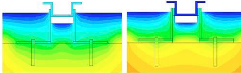
Temperature distribution of aluminum bracket without (left) and with (right) a thermostop (thermal separator)
