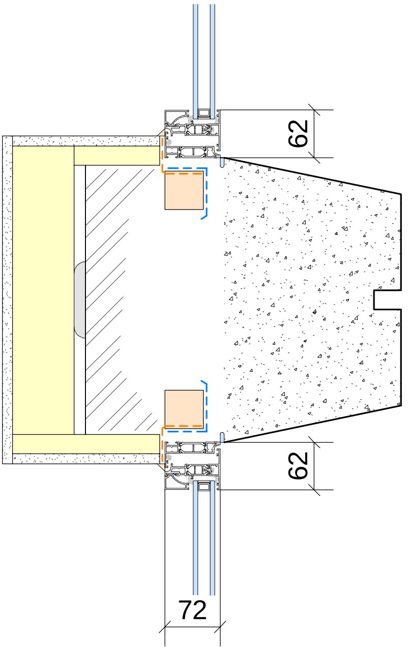
Proposed Kawneer AA720 window frame
