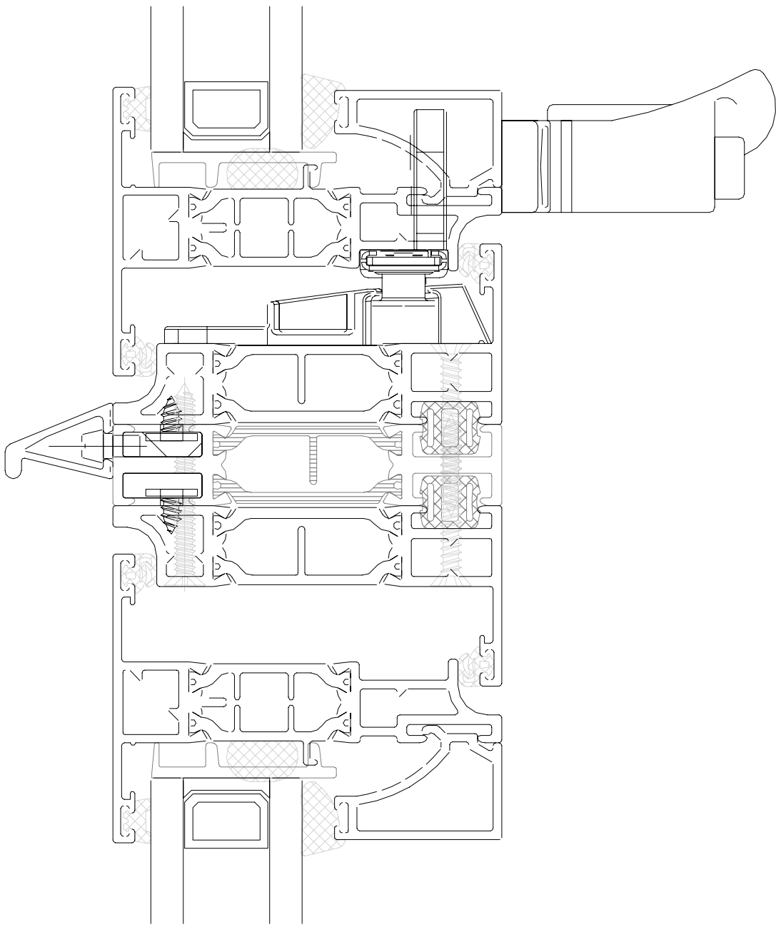
Proposed Coupling Detail
