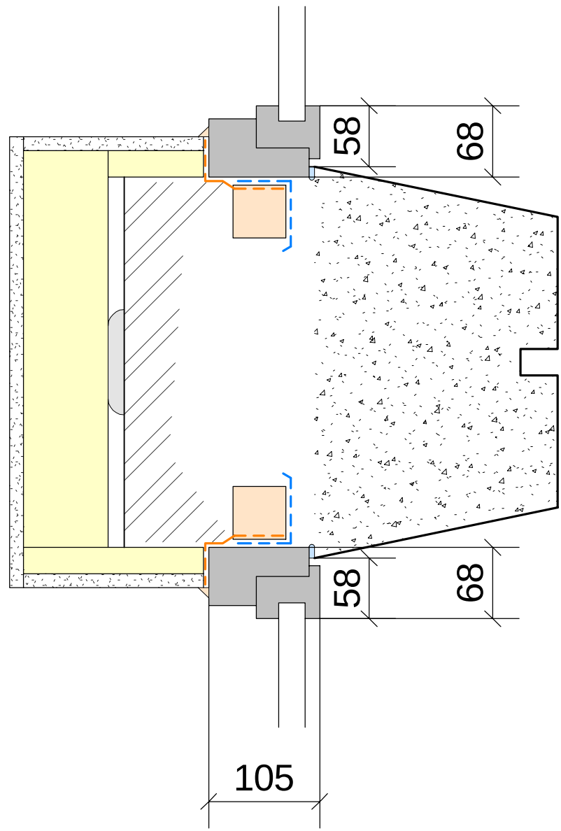
Existing Window Frame
