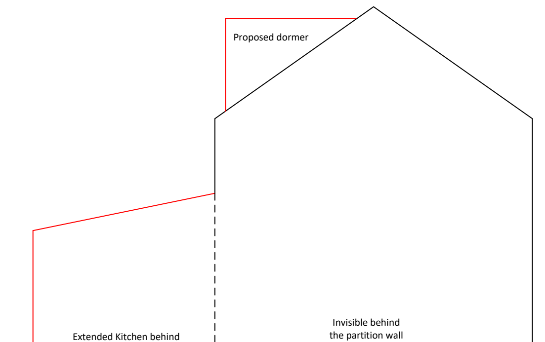
PROPOSED SIDE ELEVATION from H. No. 22
