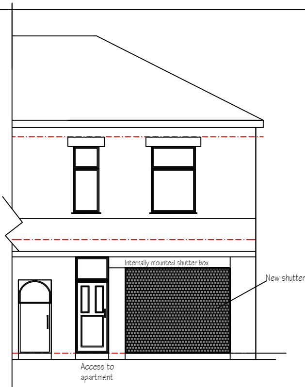
Front Elevation Showing Shop Front
