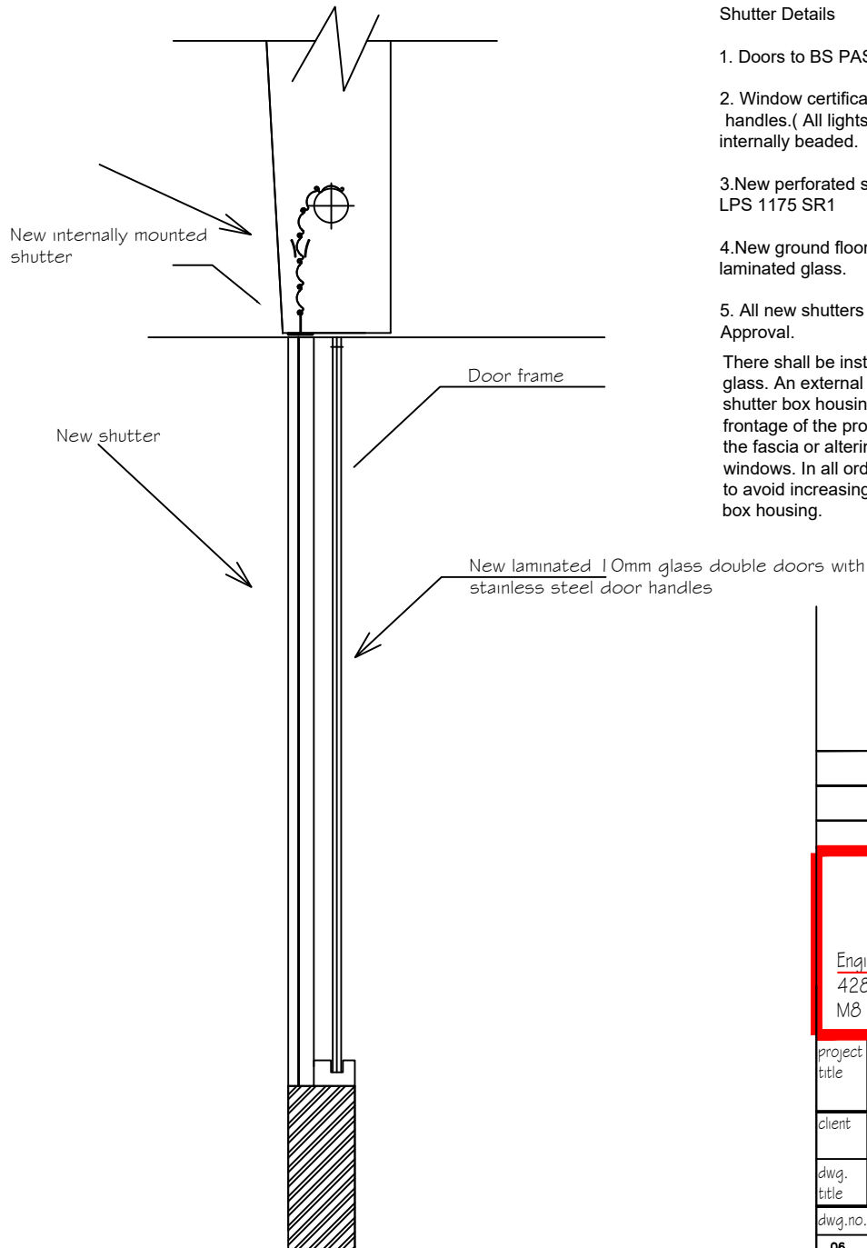
Vertical Section Showing the window and shutter details NTS
