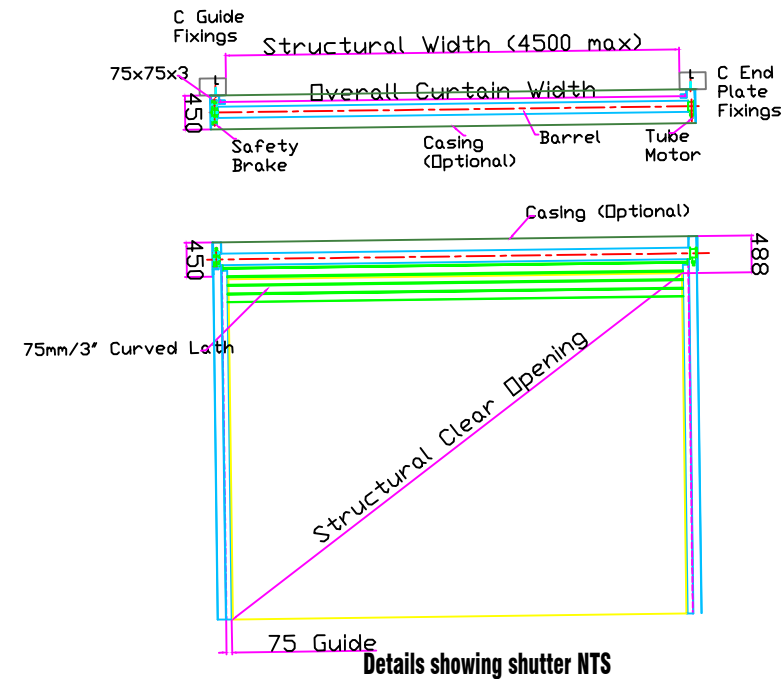
Details showing shutter NTS
