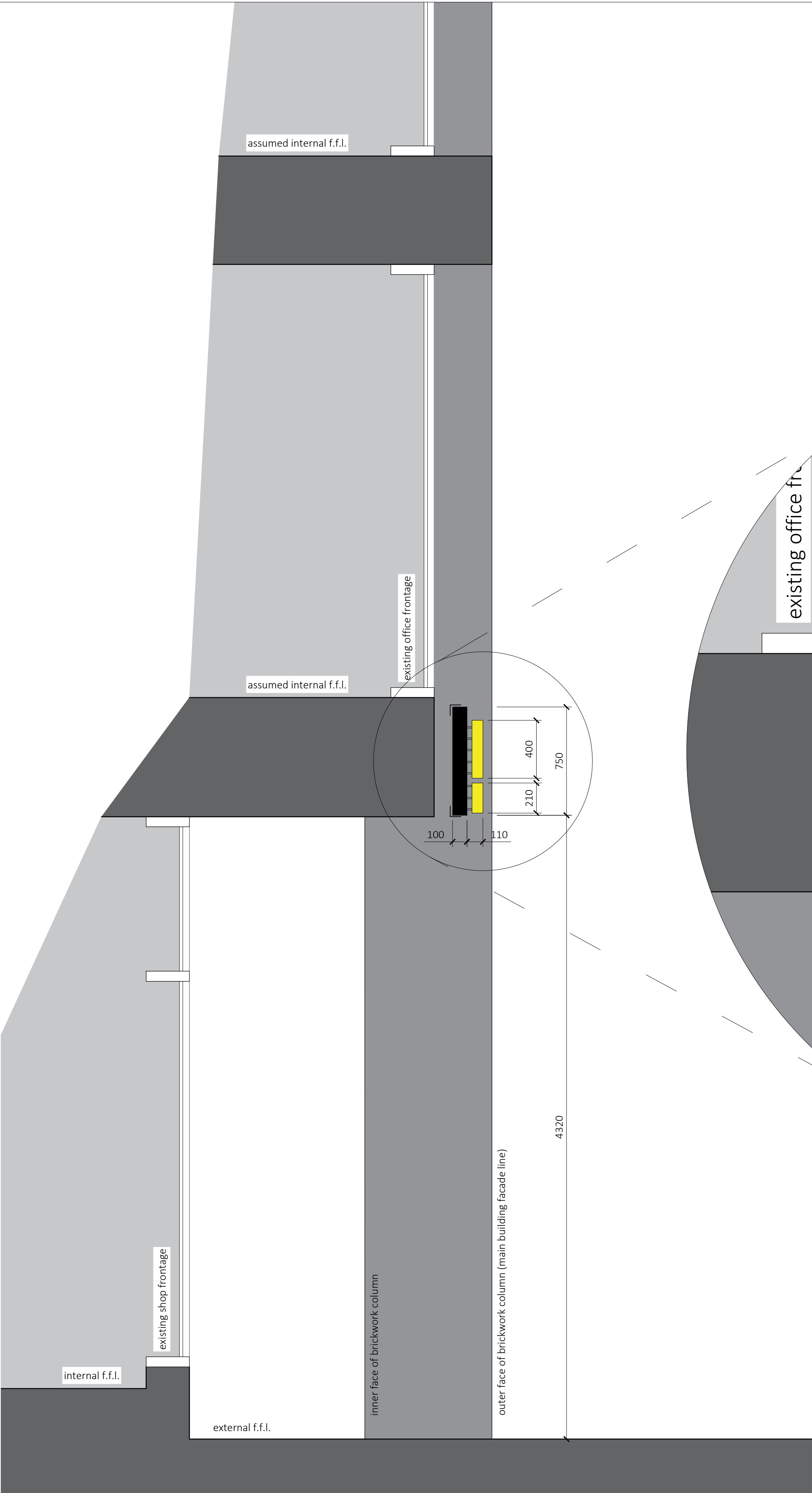
PROPOSED SECTION 1:20
