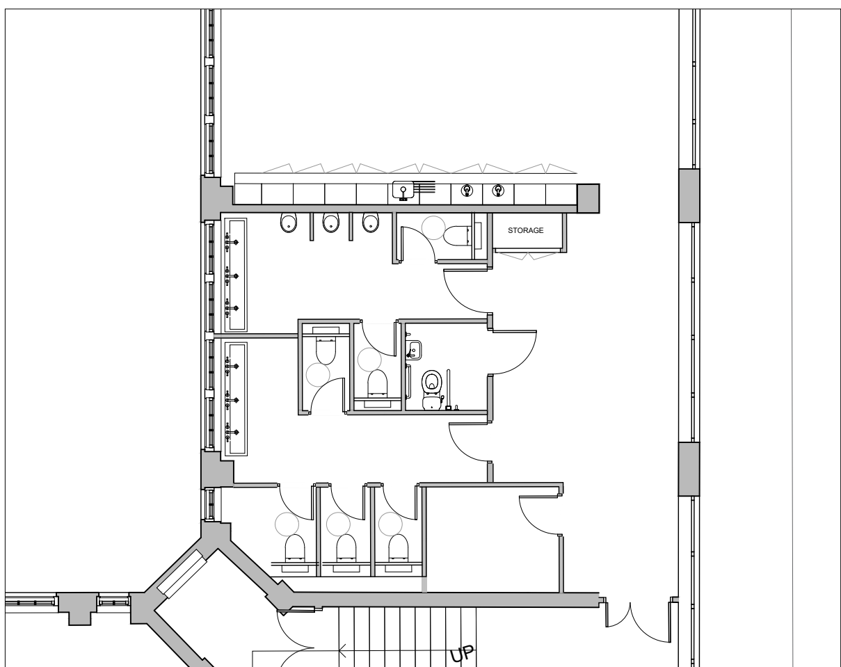
Level 13 WC - 1:100
