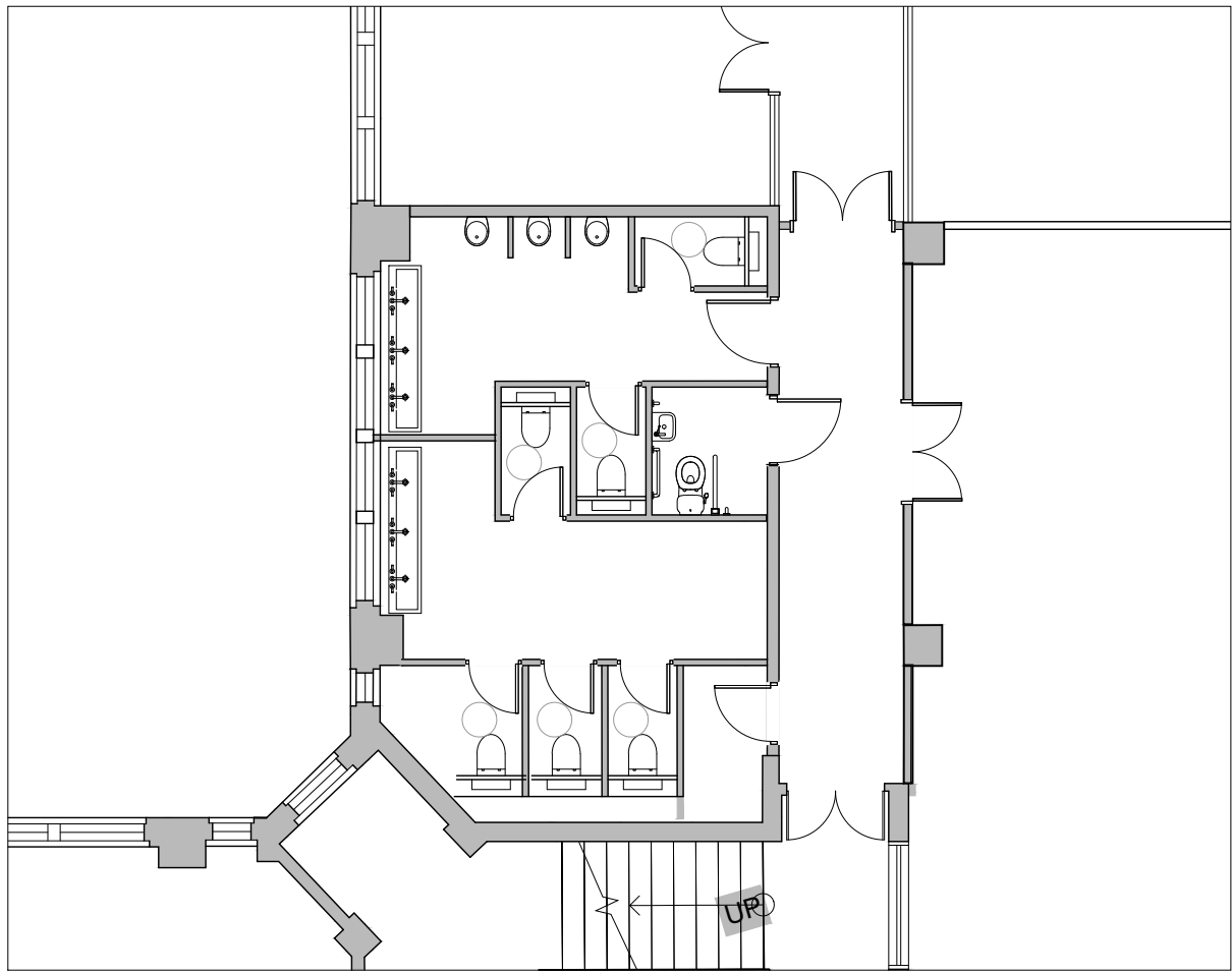
Level 02 WC - 1:100
