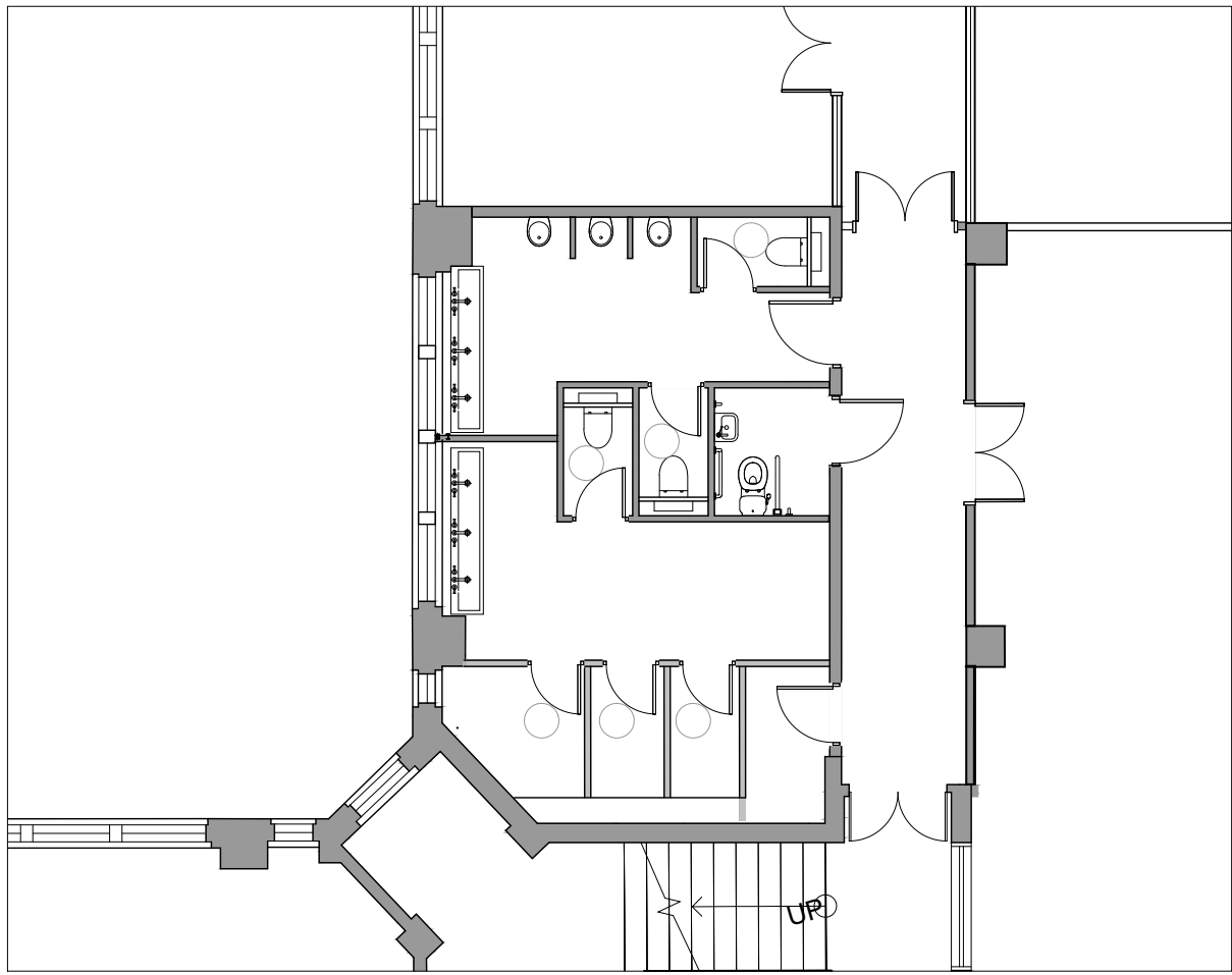
Level 03 WC - 1:100
