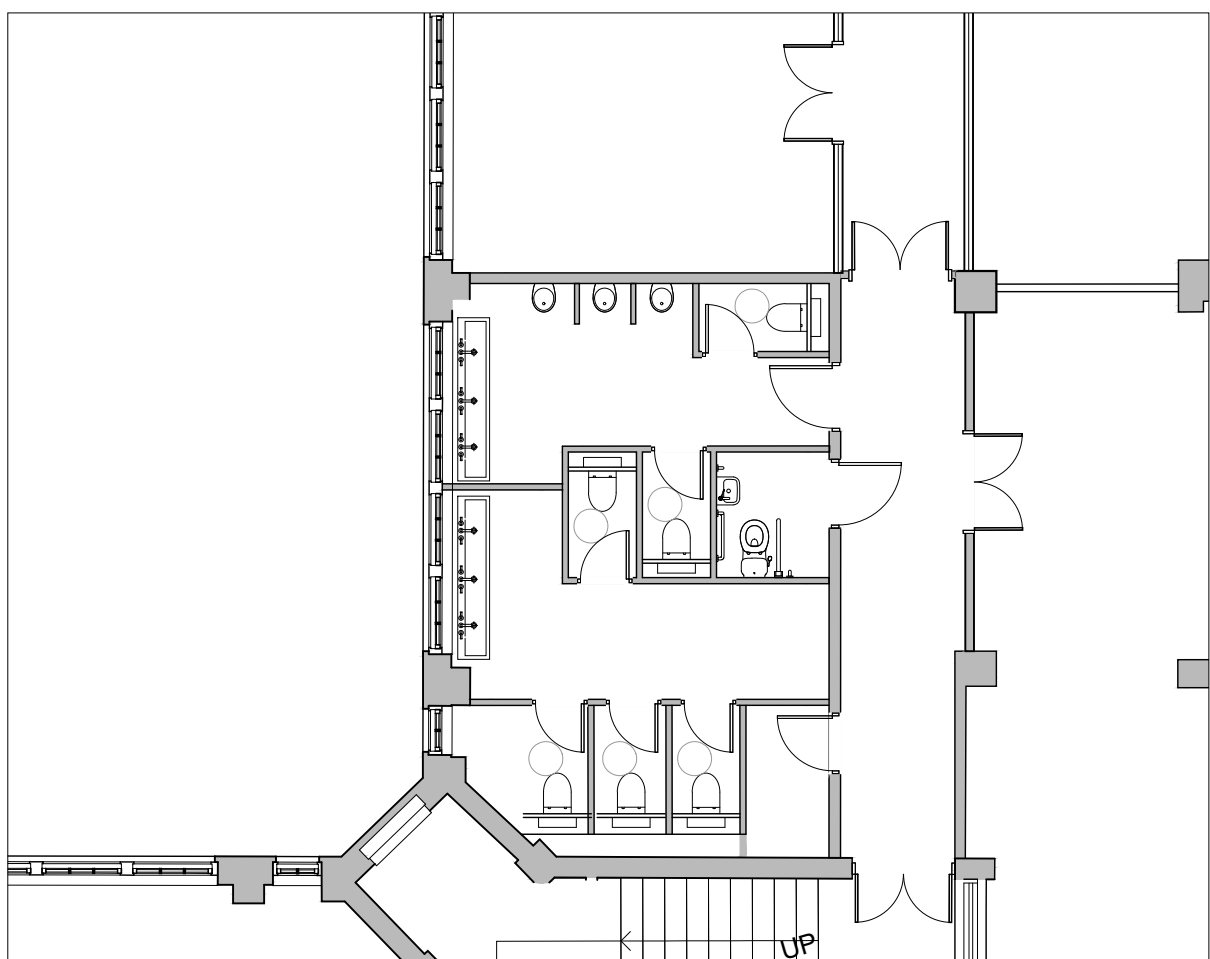
Level 12 WC - 1:100
