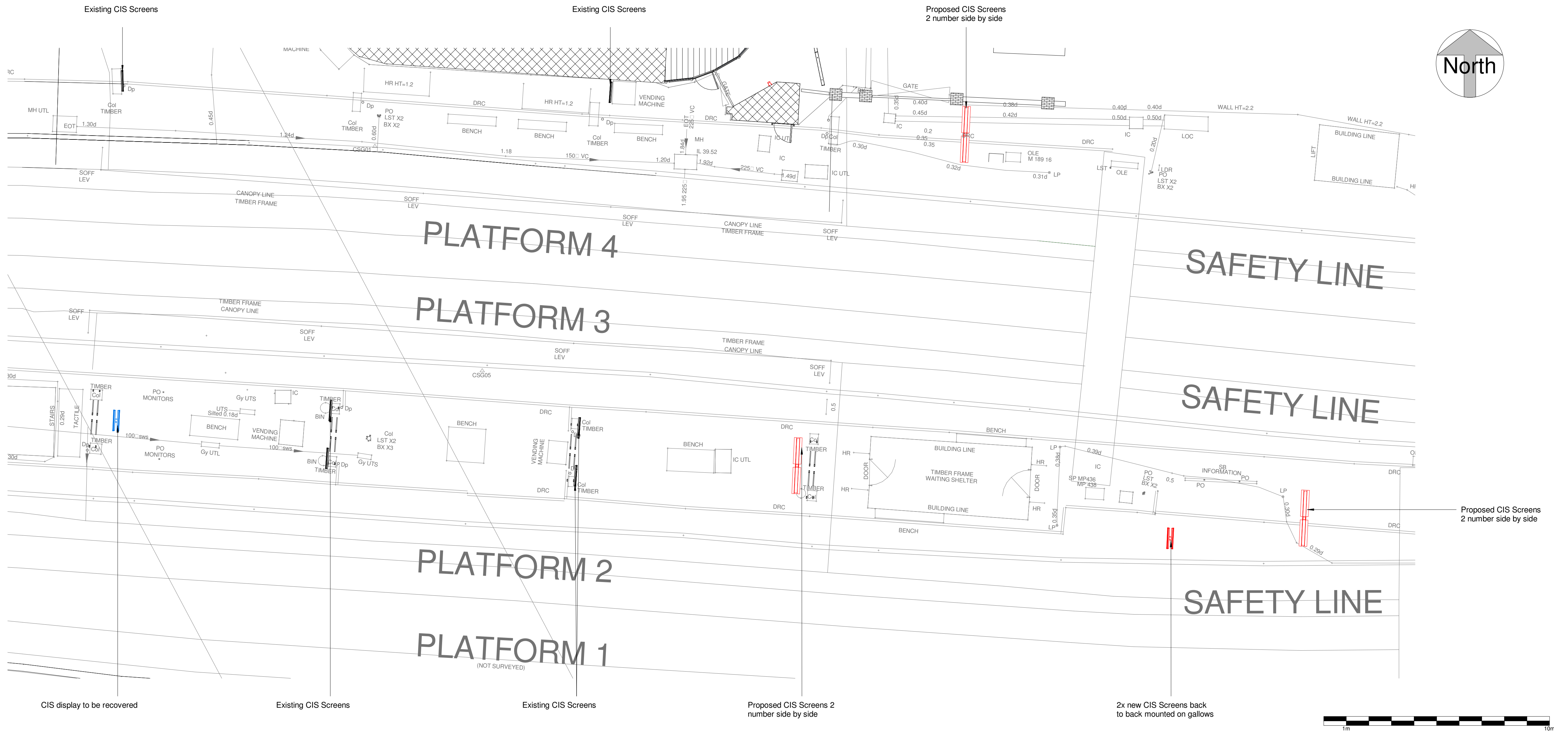
1 Proposed Ground Floor P4, P3, P2 1 : 100
