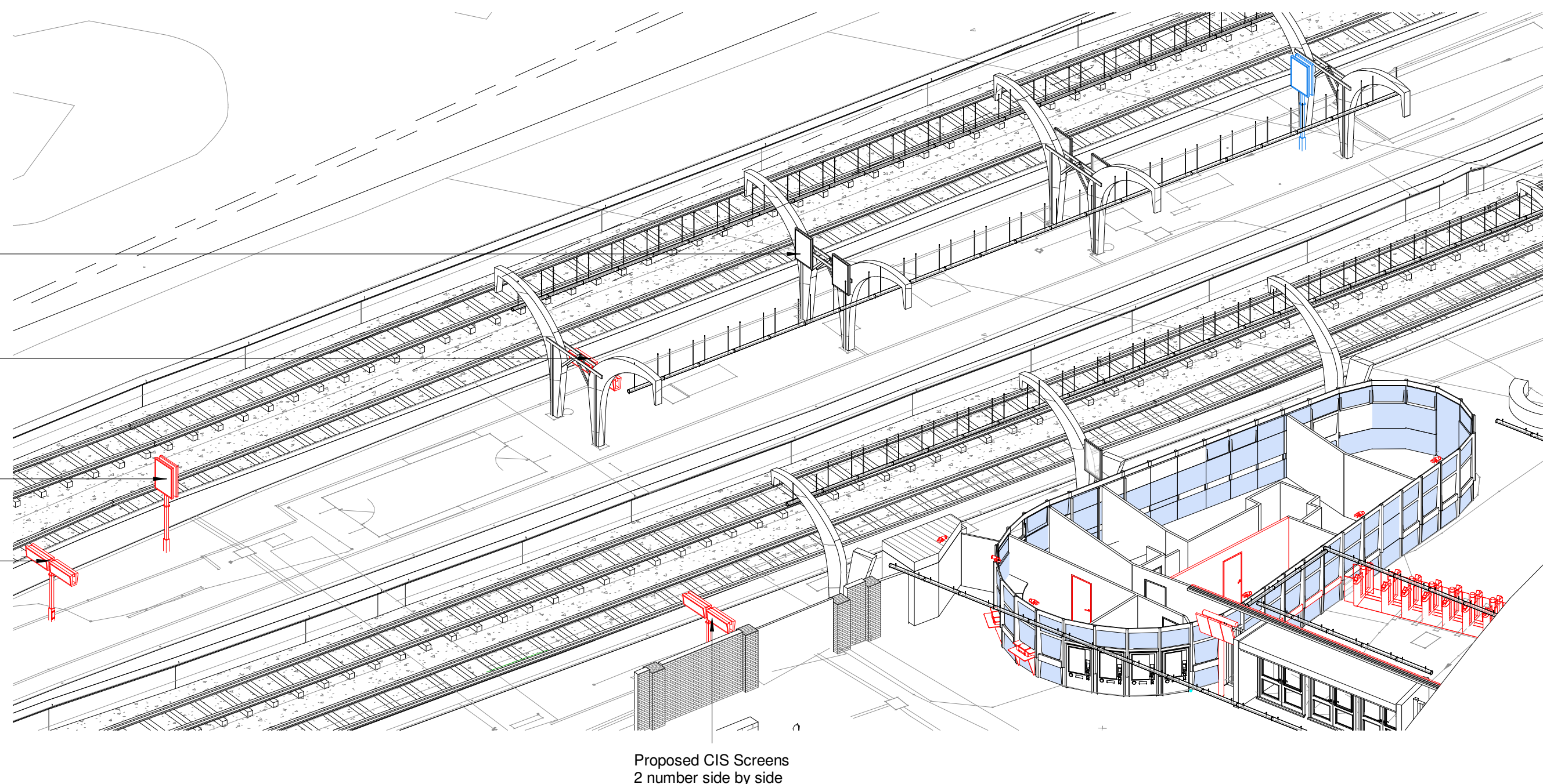
2 3D View - Showing Platform 4,3 & 2
