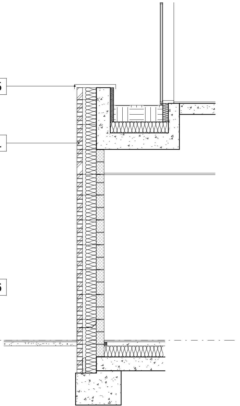
Section AA Scale 1:20 @ A1
