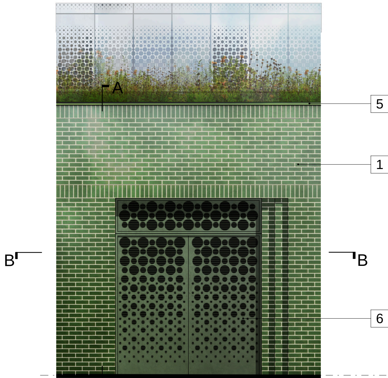
Detailed Elevation Scale 1:20 @ A1
