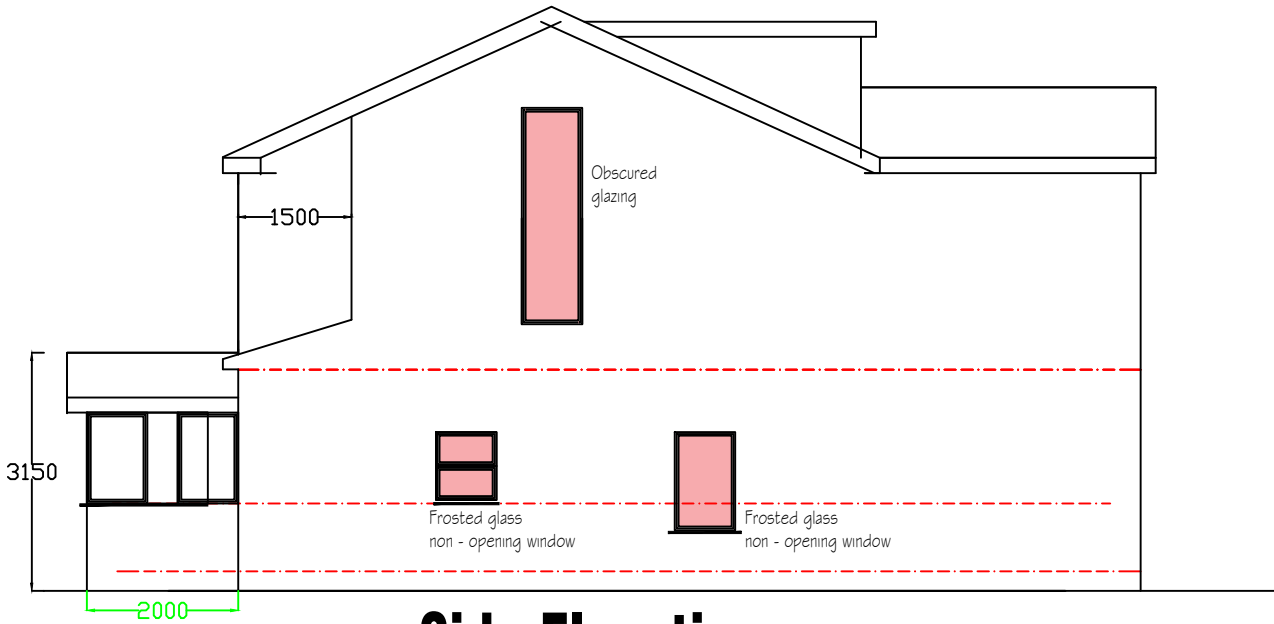
Side Elevation
