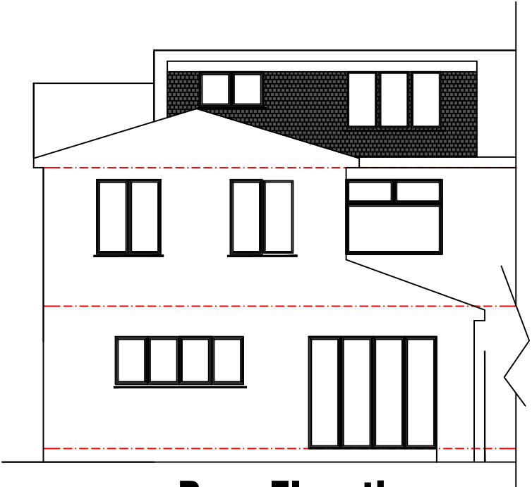
Rear Elevation
