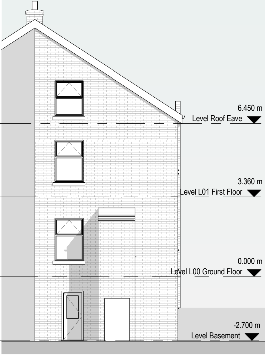
2 Existing North Elevation 1 : 100
